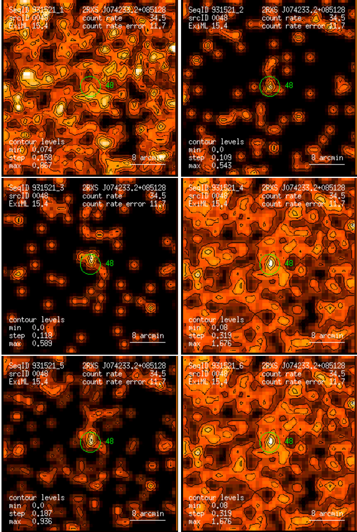
Figure 48: RASS 931521: detection 0048: band rate images, Gaussian filter: (1) PSPC channels 11 – 41, (2) 52 – 90, (3) 91 – 201, (4) 11 – 235, (5) 52 – 201, (6) 11 – 201. Broad band rates in counts/ks. Band rate contour levels in counts/ks/arcmin 2 .
