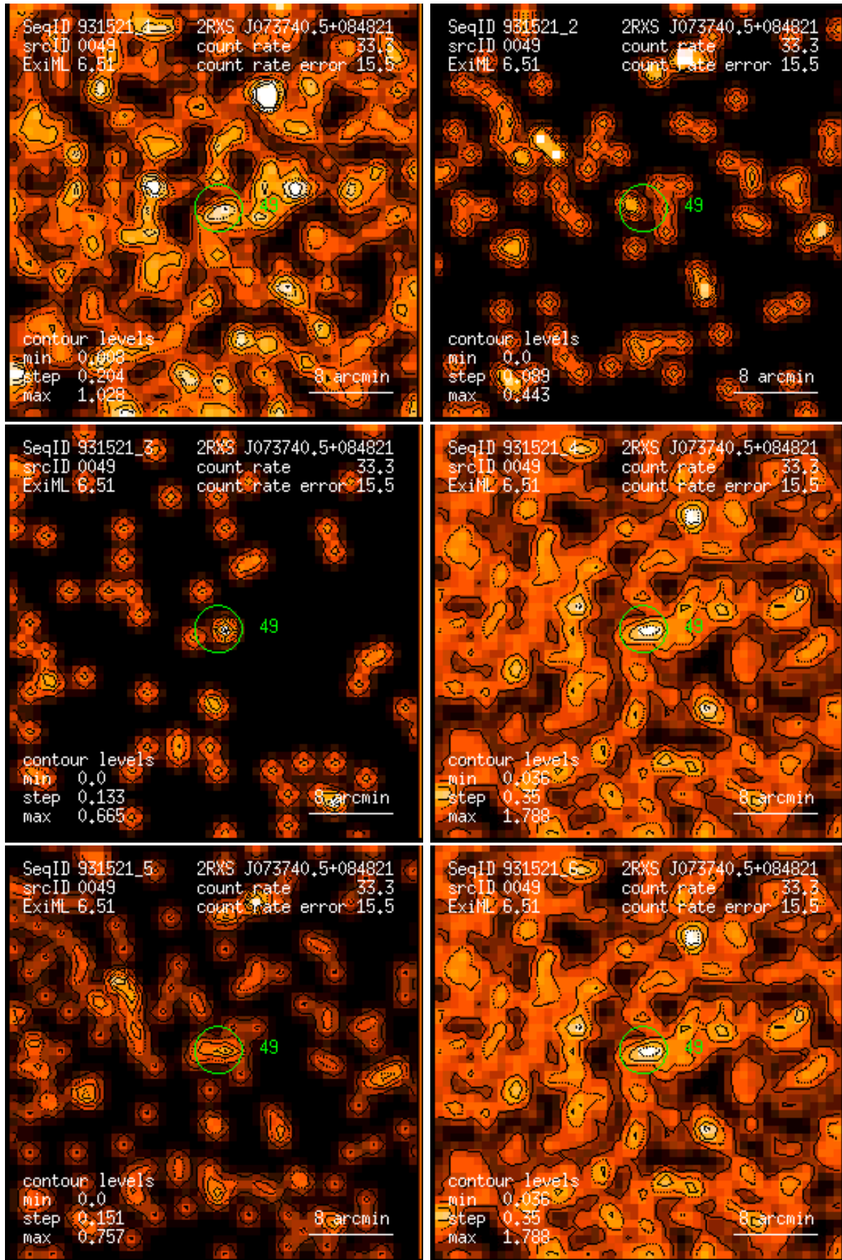
Figure 49: RASS 931521: detection 0049: band rate images, Gaussian filter: (1) PSPC channels 11 – 41, (2) 52 – 90, (3) 91 – 201, (4) 11 – 235, (5) 52 – 201, (6) 11 – 201. Broad band rates in counts/ks. Band rate contour levels in counts/ks/arcmin 2 .
