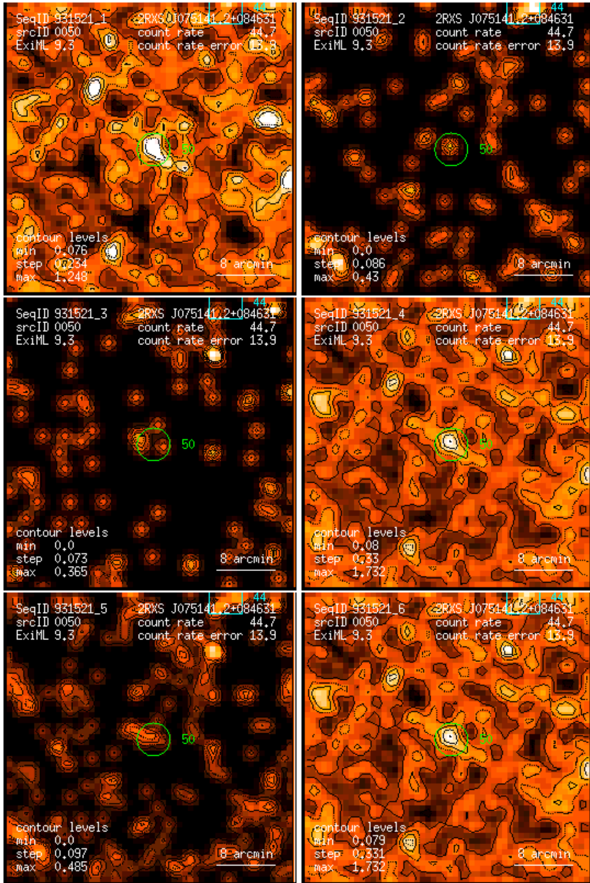
Figure 50: RASS 931521: detection 0050: band rate images, Gaussian filter: (1) PSPC channels 11 – 41, (2) 52 – 90, (3) 91 – 201, (4) 11 – 235, (5) 52 – 201, (6) 11 – 201. Broad band rates in counts/ks. Band rate contour levels in counts/ks/arcmin 2 .
