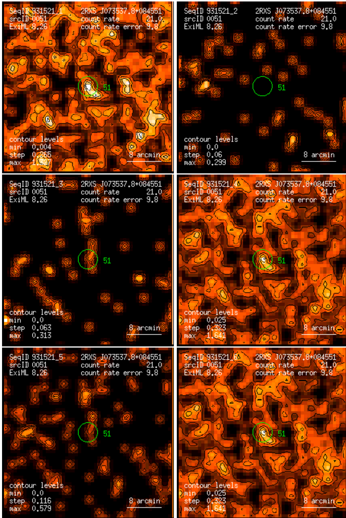
Figure 51: RASS 931521: detection 0051: band rate images, Gaussian filter: (1) PSPC channels 11 – 41, (2) 52 – 90, (3) 91 – 201, (4) 11 – 235, (5) 52 – 201, (6) 11 – 201. Broad band rates in counts/ks. Band rate contour levels in counts/ks/arcmin 2 .
