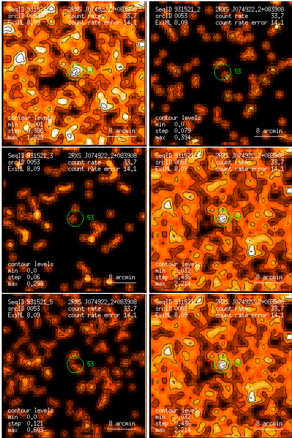
Figure 53: RASS 931521: detection 0053: band rate images, Gaussian filter: (1) PSPC channels 11 – 41, (2) 52 – 90, (3) 91 – 201, (4) 11 – 235, (5) 52 – 201, (6) 11 – 201. Broad band rates in counts/ks. Band rate contour levels in counts/ks/arcmin 2 .
