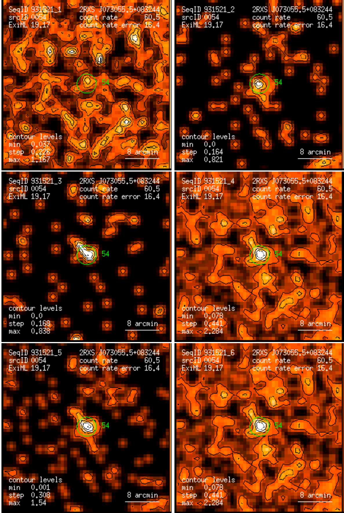
Figure 54: RASS 931521: detection 0054: band rate images, Gaussian filter: (1) PSPC channels 11 – 41, (2) 52 – 90, (3) 91 – 201, (4) 11 – 235, (5) 52 – 201, (6) 11 – 201. Broad band rates in counts/ks. Band rate contour levels in counts/ks/arcmin 2 .
