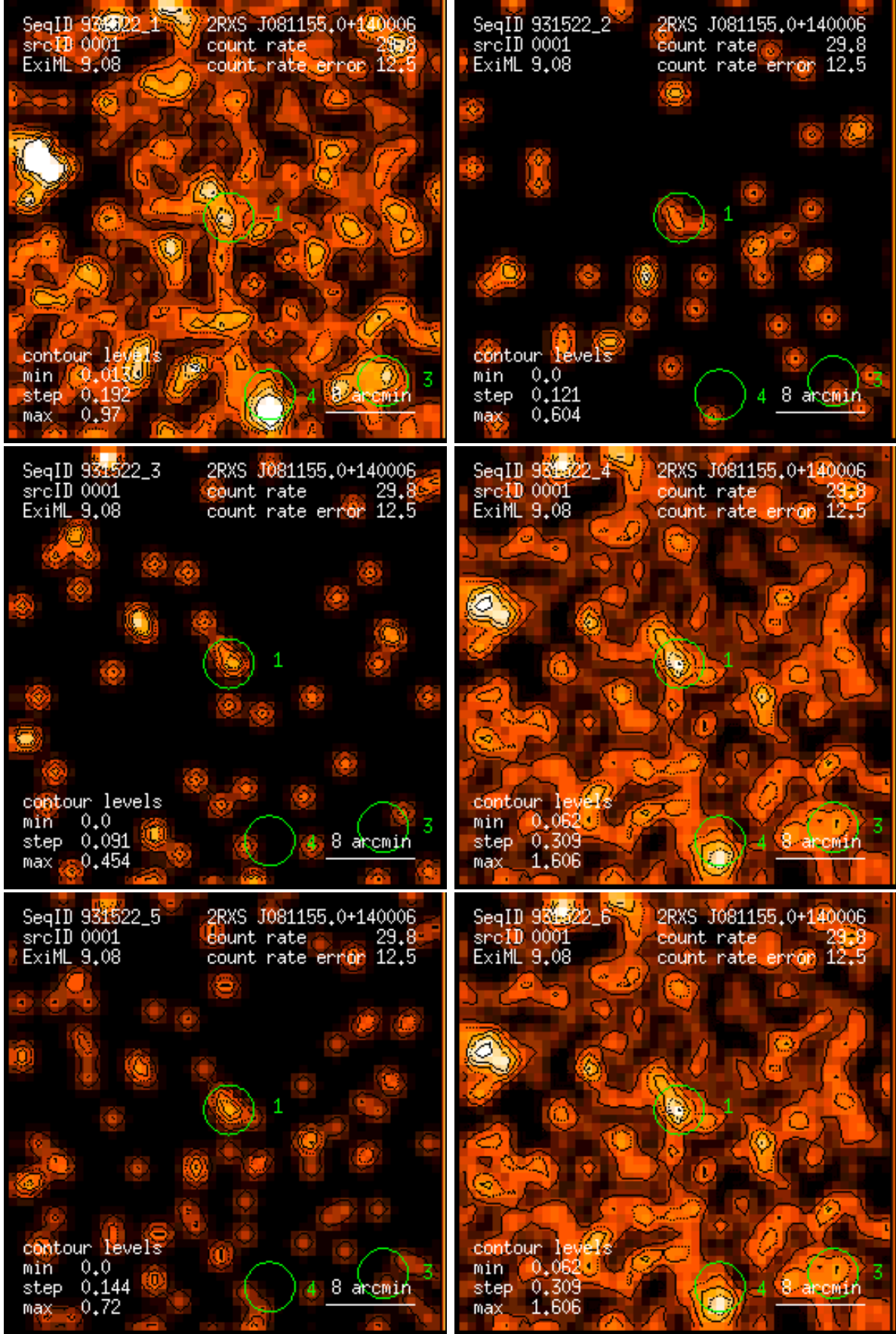
Figure 1: RASS 931522: detection 0001: band rate images, Gaussian filter: (1) PSPC channels 11 – 41, (2) 52 – 90, (3) 91 – 201, (4) 11 – 235, (5) 52 – 201, (6) 11 – 201. Broad band rates in counts/ks. Band rate contour levels in counts/ks/arcmin 2 .
