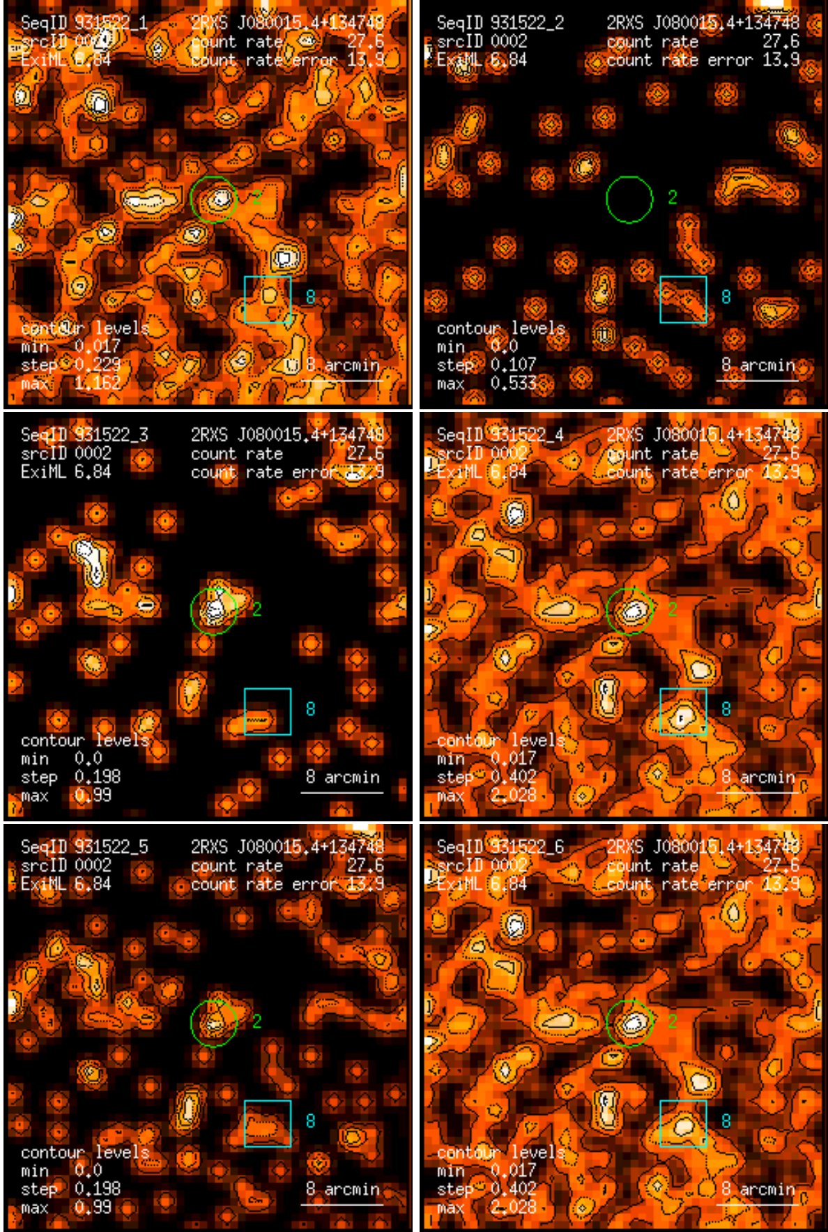
Figure 2: RASS 931522: detection 0002: band rate images, Gaussian filter: (1) PSPC channels 11 – 41, (2) 52 – 90, (3) 91 – 201, (4) 11 – 235, (5) 52 – 201, (6) 11 – 201. Broad band rates in counts/ks. Band rate contour levels in counts/ks/arcmin 2 .
