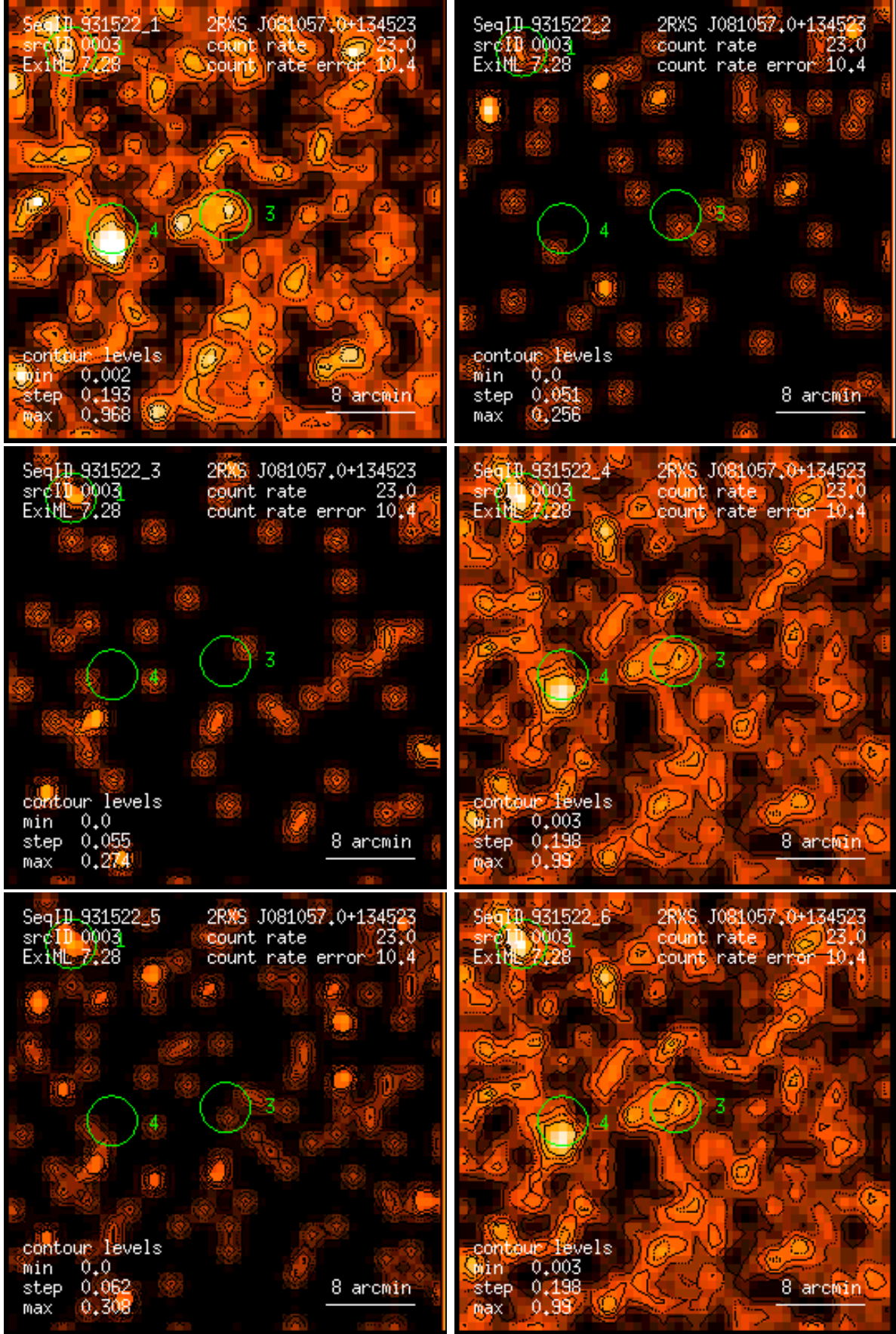
Figure 3: RASS 931522: detection 0003: band rate images, Gaussian filter: (1) PSPC channels 11 – 41, (2) 52 – 90, (3) 91 – 201, (4) 11 – 235, (5) 52 – 201, (6) 11 – 201. Broad band rates in counts/ks. Band rate contour levels in counts/ks/arcmin 2 .
