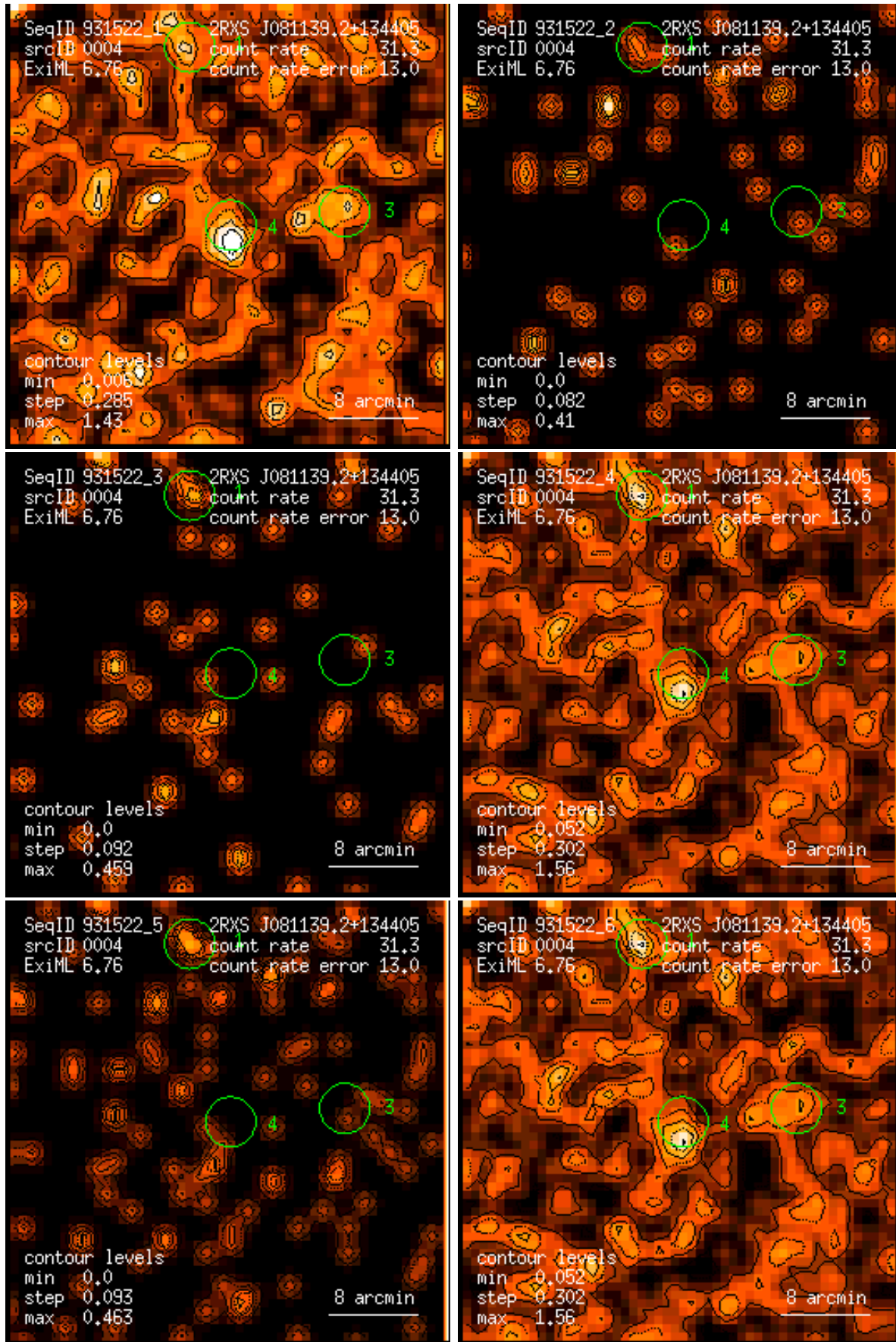
Figure 4: RASS 931522: detection 0004: band rate images, Gaussian filter: (1) PSPC channels 11 – 41, (2) 52 – 90, (3) 91 – 201, (4) 11 – 235, (5) 52 – 201, (6) 11 – 201. Broad band rates in counts/ks. Band rate contour levels in counts/ks/arcmin 2 .
