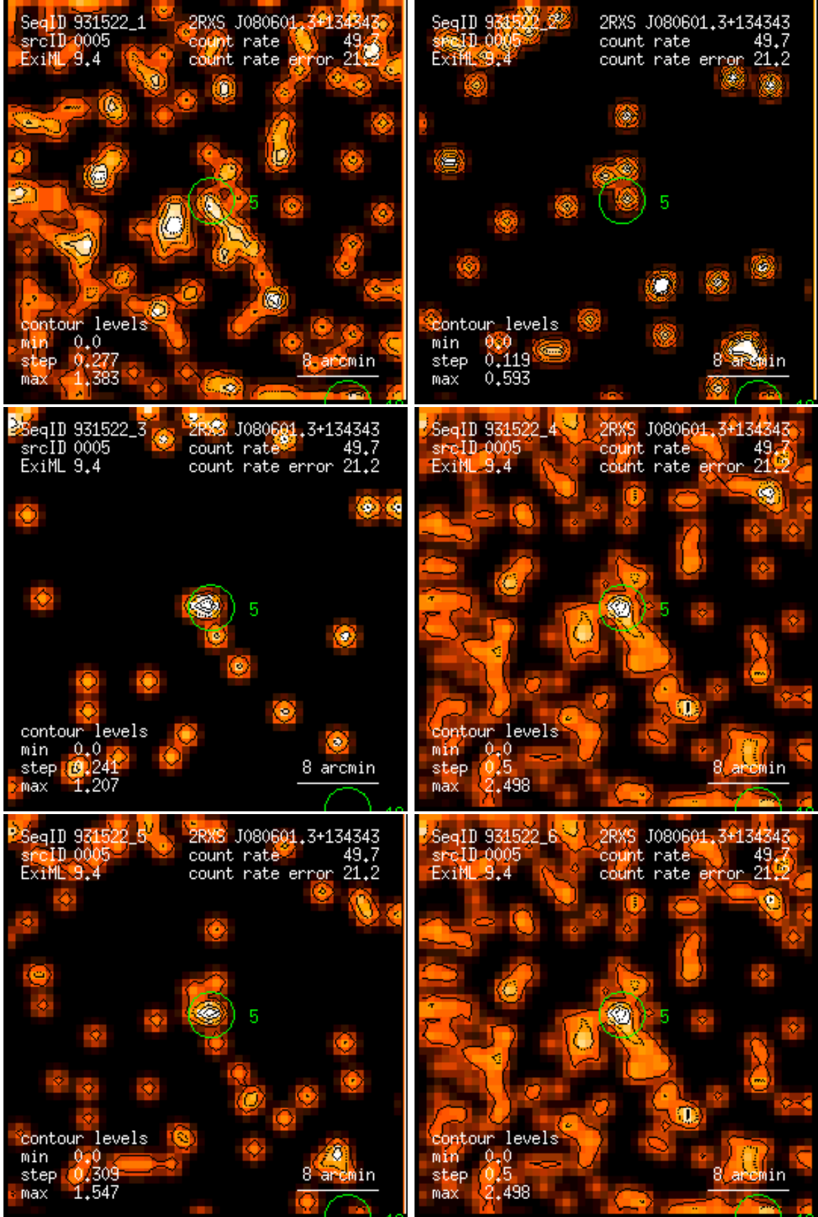
Figure 5: RASS 931522: detection 0005: band rate images, Gaussian filter: (1) PSPC channels 11 – 41, (2) 52 – 90, (3) 91 – 201, (4) 11 – 235, (5) 52 – 201, (6) 11 – 201. Broad band rates in counts/ks. Band rate contour levels in counts/ks/arcmin 2 .
