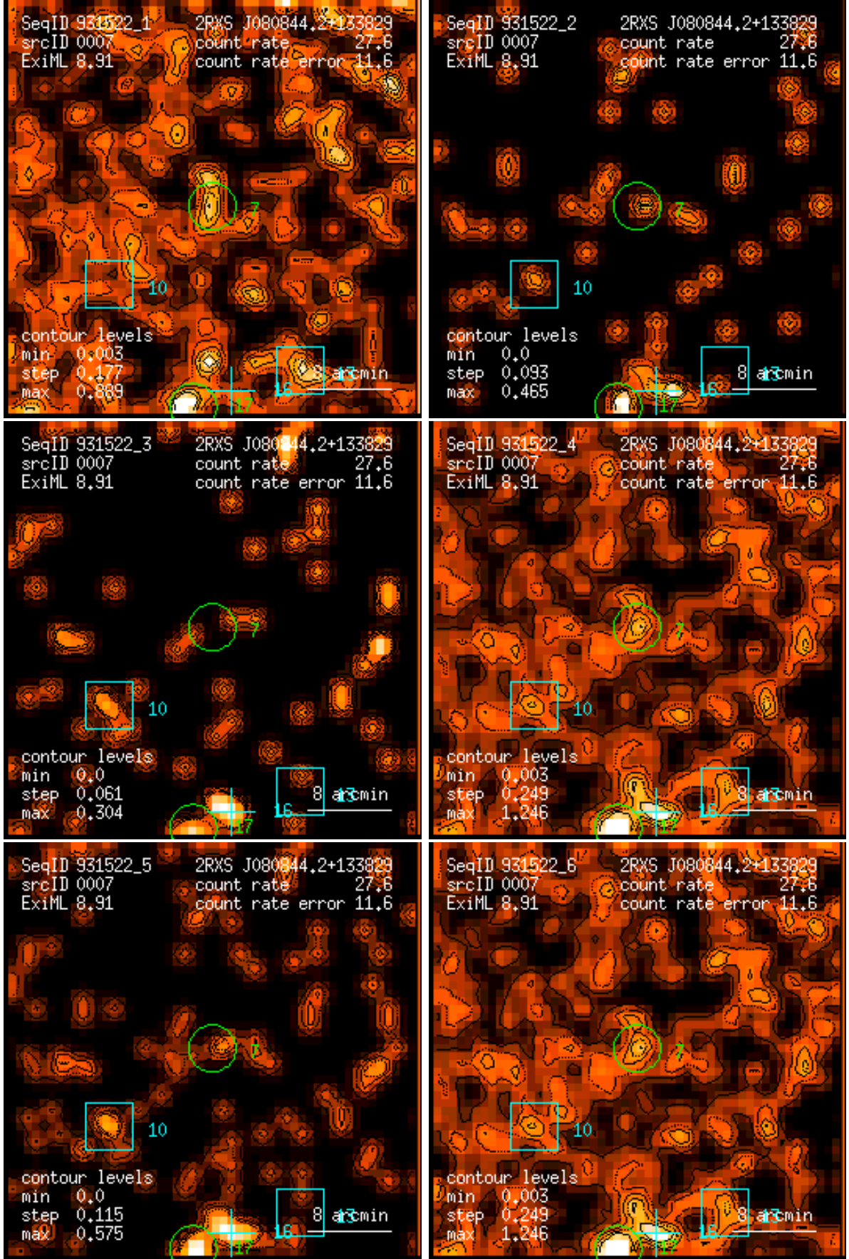
Figure 7: RASS 931522: detection 0007: band rate images, Gaussian filter: (1) PSPC channels 11 – 41, (2) 52 – 90, (3) 91 – 201, (4) 11 – 235, (5) 52 – 201, (6) 11 – 201. Broad band rates in counts/ks. Band rate contour levels in counts/ks/arcmin 2 .
