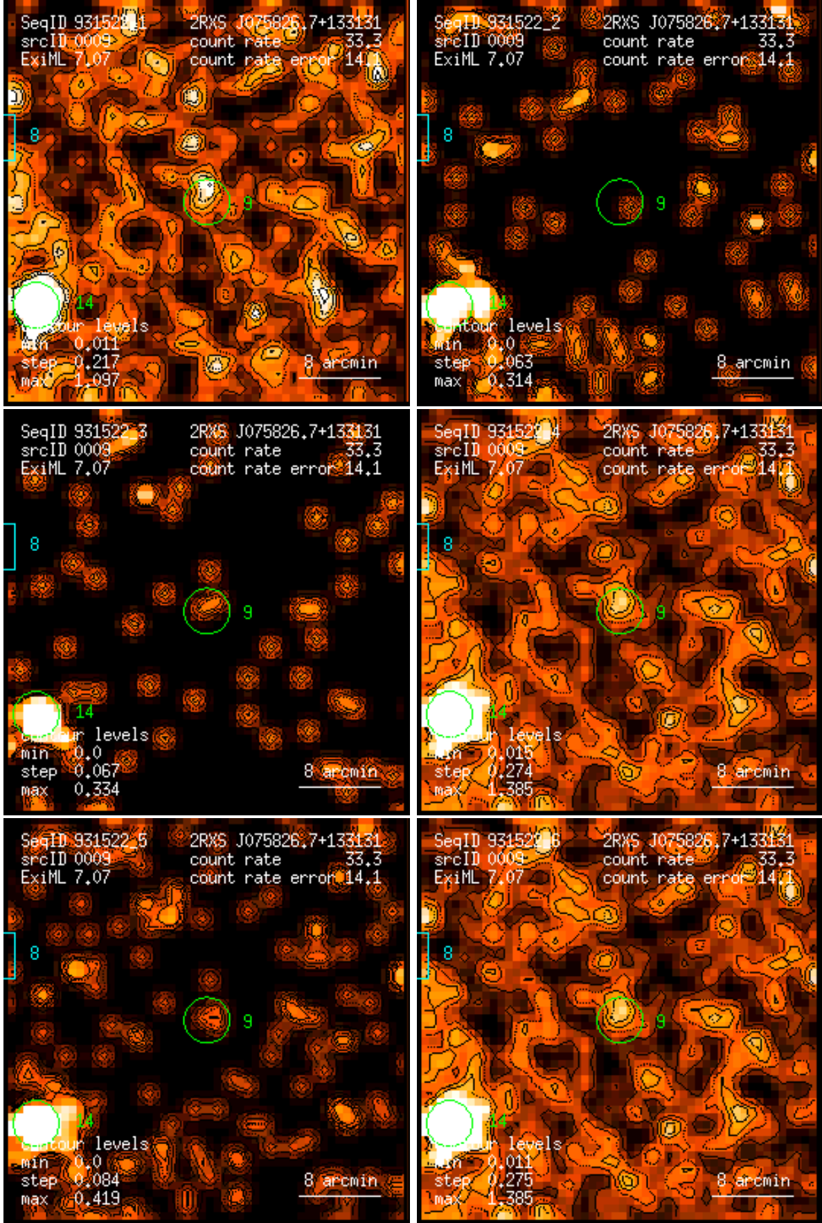
Figure 9: RASS 931522: detection 0009: band rate images, Gaussian filter: (1) PSPC channels 11 – 41, (2) 52 – 90, (3) 91 – 201, (4) 11 – 235, (5) 52 – 201, (6) 11 – 201. Broad band rates in counts/ks. Band rate contour levels in counts/ks/arcmin 2 .
