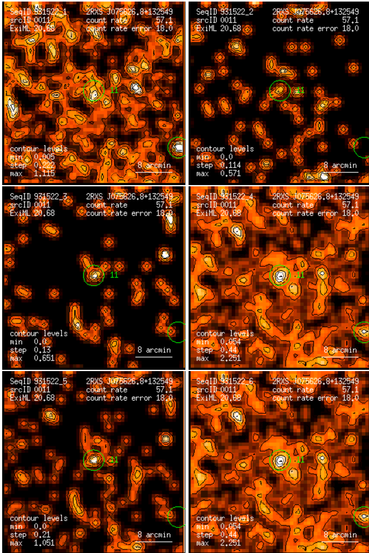
Figure 11: RASS 931522: detection 0011: band rate images, Gaussian filter: (1) PSPC channels 11 – 41, (2) 52 – 90, (3) 91 – 201, (4) 11 – 235, (5) 52 – 201, (6) 11 – 201. Broad band rates in counts/ks. Band rate contour levels in counts/ks/arcmin 2 .
