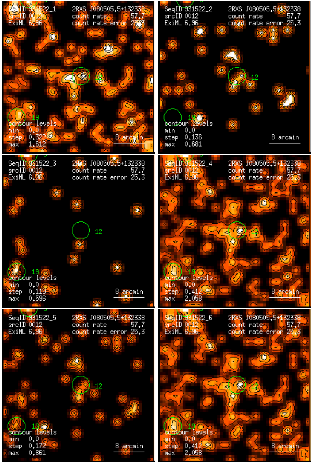
Figure 12: RASS 931522: detection 0012: band rate images, Gaussian filter: (1) PSPC channels 11 – 41, (2) 52 – 90, (3) 91 – 201, (4) 11 – 235, (5) 52 – 201, (6) 11 – 201. Broad band rates in counts/ks. Band rate contour levels in counts/ks/arcmin 2 .
