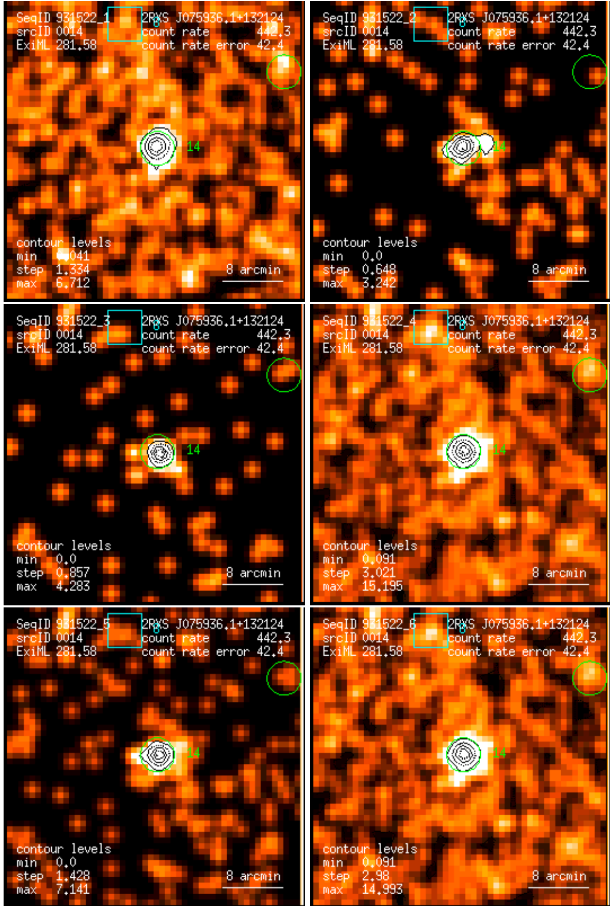
Figure 14: RASS 931522: detection 0014: band rate images, Gaussian filter: (1) PSPC channels 11 – 41, (2) 52 – 90, (3) 91 – 201, (4) 11 – 235, (5) 52 – 201, (6) 11 – 201. Broad band rates in counts/ks. Band rate contour levels in counts/ks/arcmin 2 .
