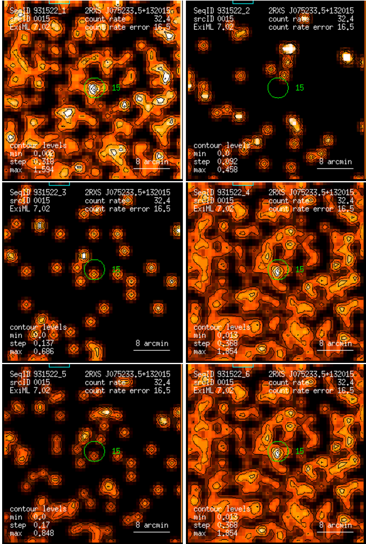
Figure 15: RASS 931522: detection 0015: band rate images, Gaussian filter: (1) PSPC channels 11 – 41, (2) 52 – 90, (3) 91 – 201, (4) 11 – 235, (5) 52 – 201, (6) 11 – 201. Broad band rates in counts/ks. Band rate contour levels in counts/ks/arcmin 2 .
