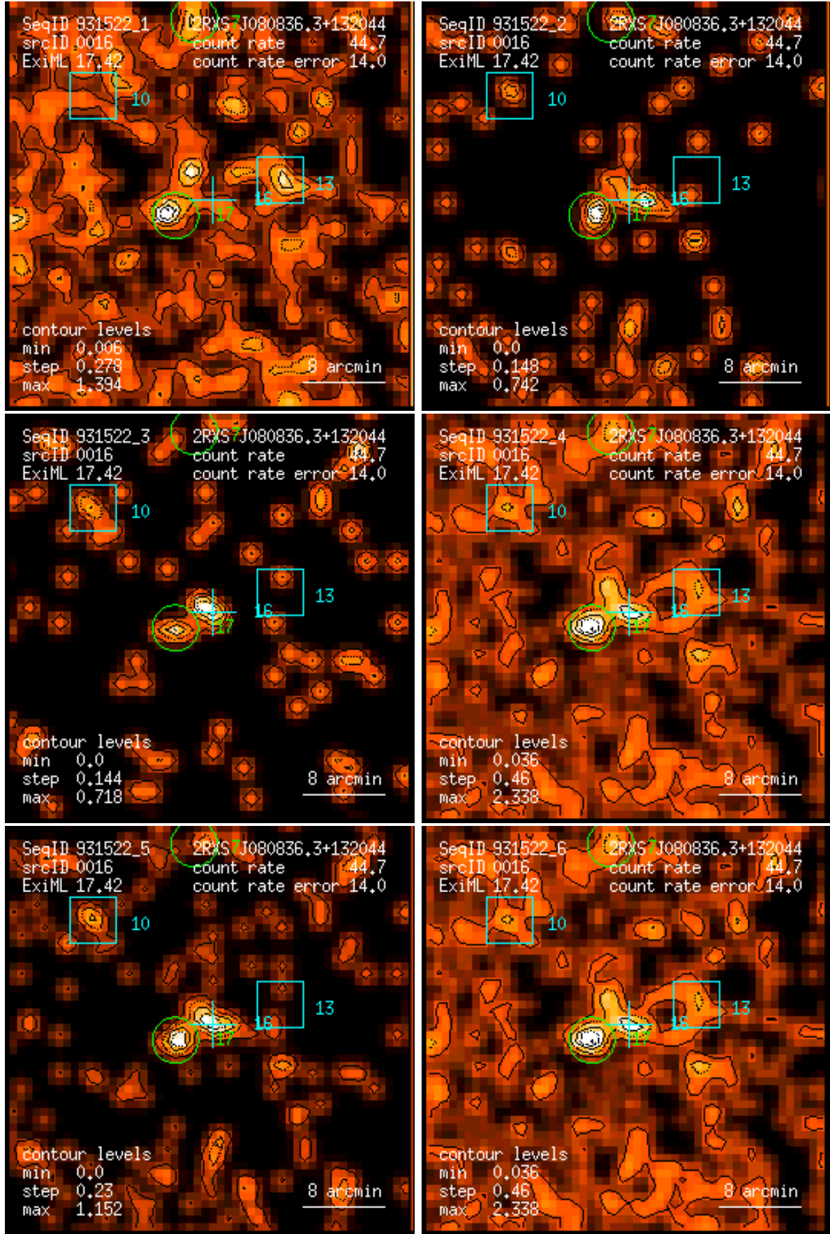
Figure 16: RASS 931522: detection 0016: band rate images, Gaussian filter: (1) PSPC channels 11 – 41, (2) 52 – 90, (3) 91 – 201, (4) 11 – 235, (5) 52 – 201, (6) 11 – 201. Broad band rates in counts/ks. Band rate contour levels in counts/ks/arcmin 2 .
