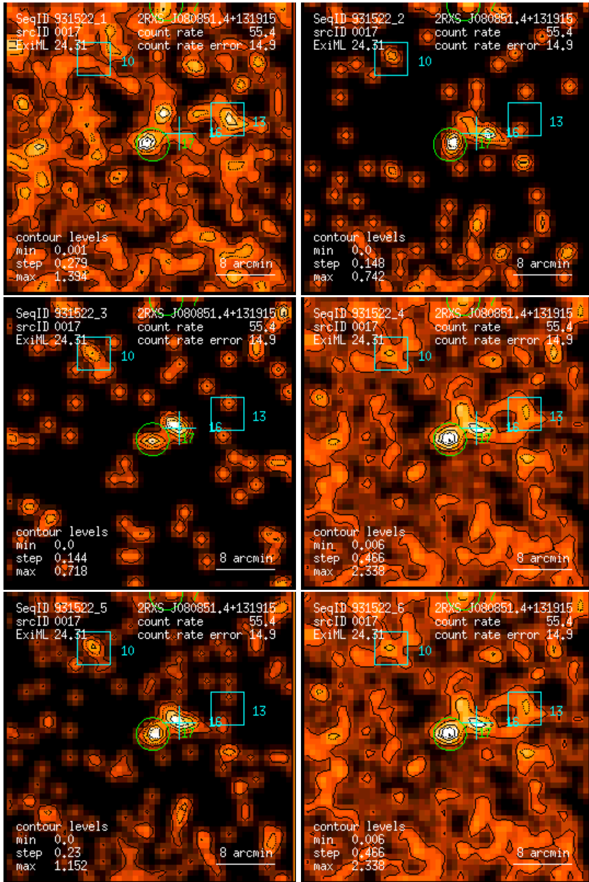
Figure 17: RASS 931522: detection 0017: band rate images, Gaussian filter: (1) PSPC channels 11 – 41, (2) 52 – 90, (3) 91 – 201, (4) 11 – 235, (5) 52 – 201, (6) 11 – 201. Broad band rates in counts/ks. Band rate contour levels in counts/ks/arcmin 2 .
