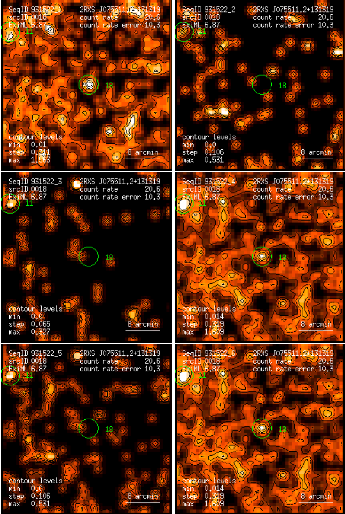
Figure 18: RASS 931522: detection 0018: band rate images, Gaussian filter: (1) PSPC channels 11 – 41, (2) 52 – 90, (3) 91 – 201, (4) 11 – 235, (5) 52 – 201, (6) 11 – 201. Broad band rates in counts/ks. Band rate contour levels in counts/ks/arcmin 2 .
