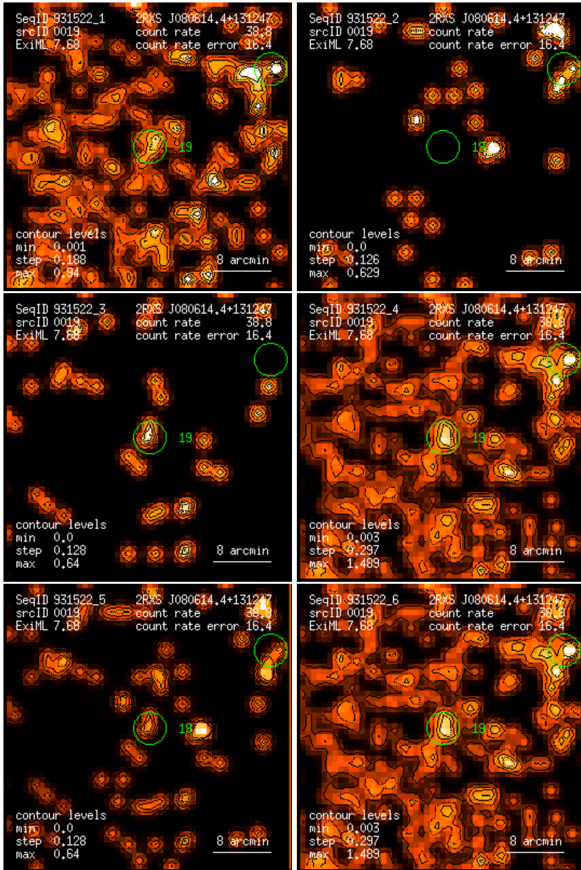
Figure 19: RASS 931522: detection 0019: band rate images, Gaussian filter: (1) PSPC channels 11 – 41, (2) 52 – 90, (3) 91 – 201, (4) 11 – 235, (5) 52 – 201, (6) 11 – 201. Broad band rates in counts/ks. Band rate contour levels in counts/ks/arcmin 2 .
