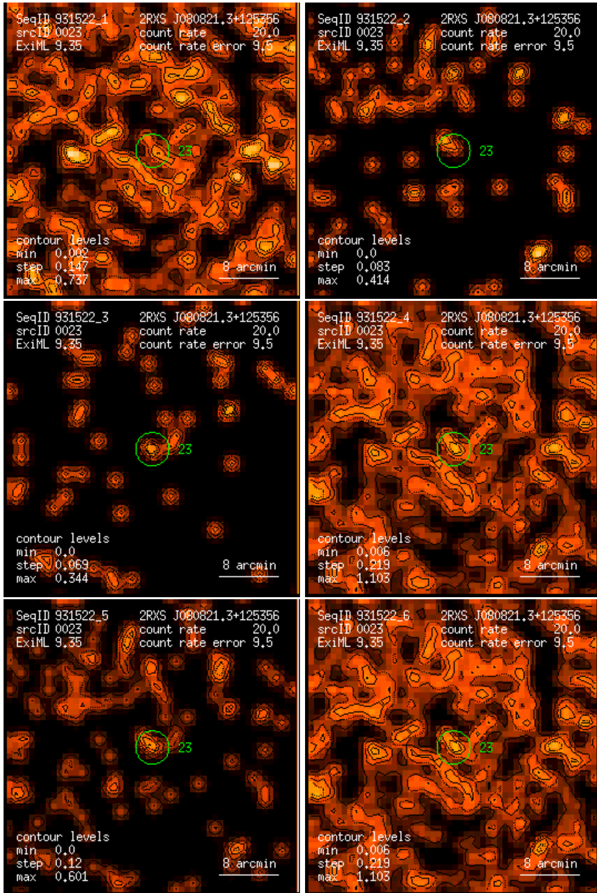
Figure 23: RASS 931522: detection 0023: band rate images, Gaussian filter: (1) PSPC channels 11 – 41, (2) 52 – 90, (3) 91 – 201, (4) 11 – 235, (5) 52 – 201, (6) 11 – 201. Broad band rates in counts/ks. Band rate contour levels in counts/ks/arcmin 2 .
