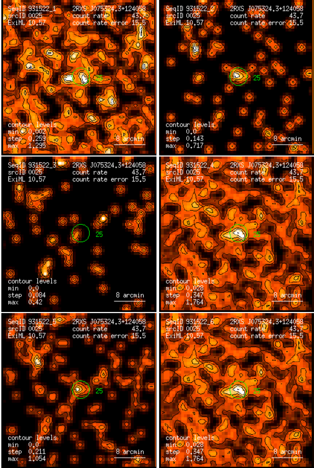
Figure 25: RASS 931522: detection 0025: band rate images, Gaussian filter: (1) PSPC channels 11 – 41, (2) 52 – 90, (3) 91 – 201, (4) 11 – 235, (5) 52 – 201, (6) 11 – 201. Broad band rates in counts/ks. Band rate contour levels in counts/ks/arcmin 2 .
