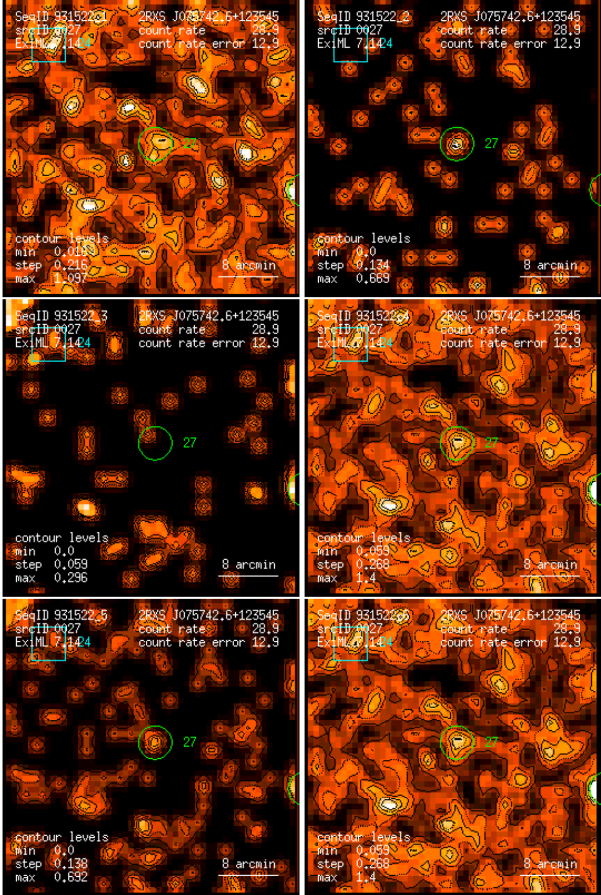
Figure 27: RASS 931522: detection 0027: band rate images, Gaussian filter: (1) PSPC channels 11 – 41, (2) 52 – 90, (3) 91 – 201, (4) 11 – 235, (5) 52 – 201, (6) 11 – 201. Broad band rates in counts/ks. Band rate contour levels in counts/ks/arcmin 2 .
