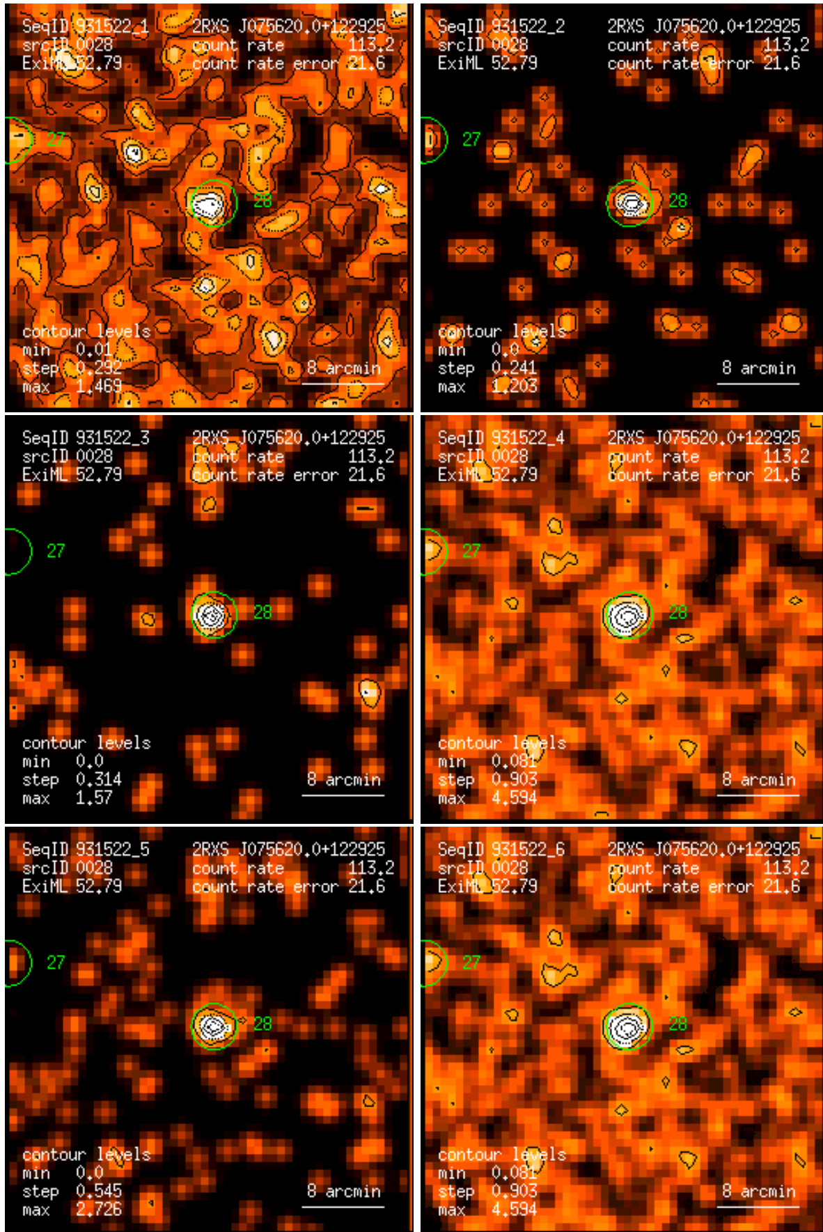
Figure 28: RASS 931522: detection 0028: band rate images, Gaussian filter: (1) PSPC channels 11 – 41, (2) 52 – 90, (3) 91 – 201, (4) 11 – 235, (5) 52 – 201, (6) 11 – 201. Broad band rates in counts/ks. Band rate contour levels in counts/ks/arcmin 2 .
