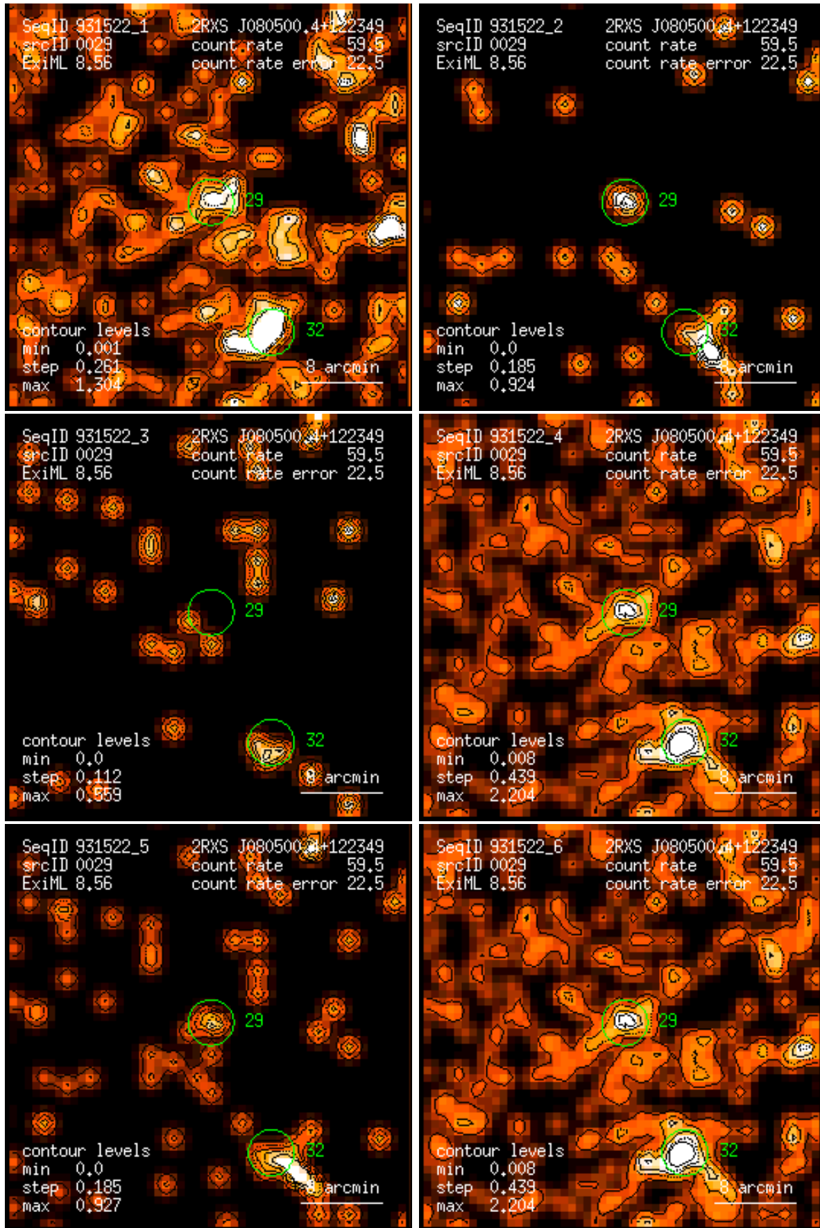
Figure 29: RASS 931522: detection 0029: band rate images, Gaussian filter: (1) PSPC channels 11 – 41, (2) 52 – 90, (3) 91 – 201, (4) 11 – 235, (5) 52 – 201, (6) 11 – 201. Broad band rates in counts/ks. Band rate contour levels in counts/ks/arcmin 2 .
