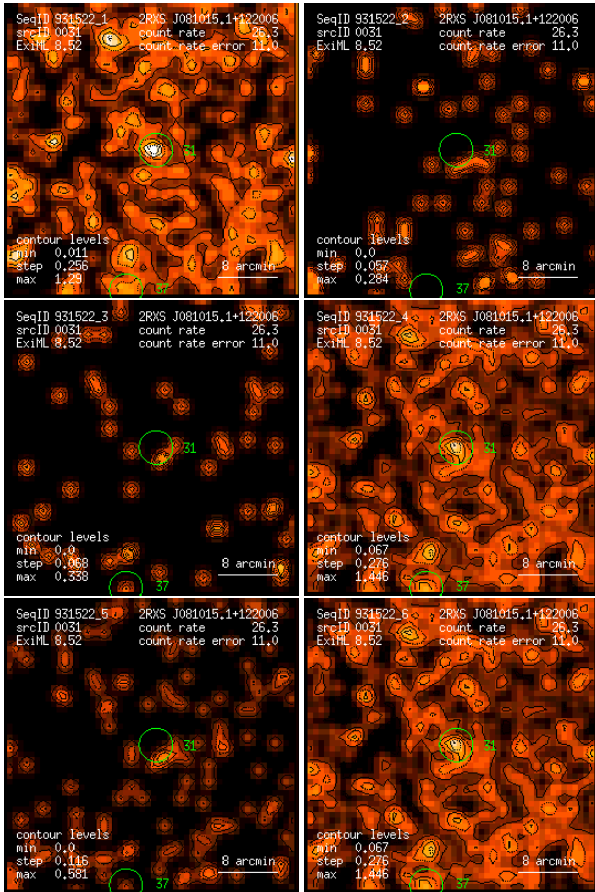
Figure 31: RASS 931522: detection 0031: band rate images, Gaussian filter: (1) PSPC channels 11 – 41, (2) 52 – 90, (3) 91 – 201, (4) 11 – 235, (5) 52 – 201, (6) 11 – 201. Broad band rates in counts/ks. Band rate contour levels in counts/ks/arcmin 2 .
