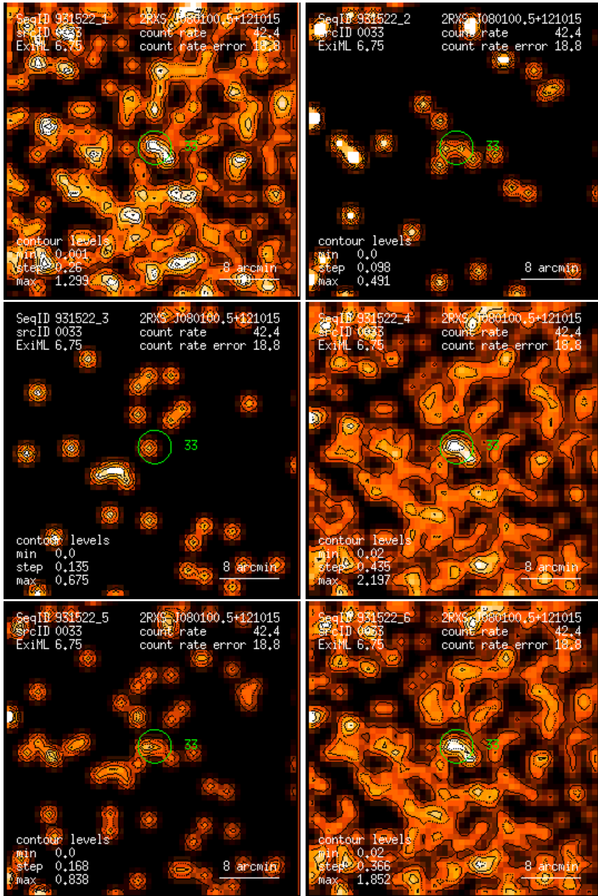
Figure 33: RASS 931522: detection 0033: band rate images, Gaussian filter: (1) PSPC channels 11 – 41, (2) 52 – 90, (3) 91 – 201, (4) 11 – 235, (5) 52 – 201, (6) 11 – 201. Broad band rates in counts/ks. Band rate contour levels in counts/ks/arcmin 2 .
