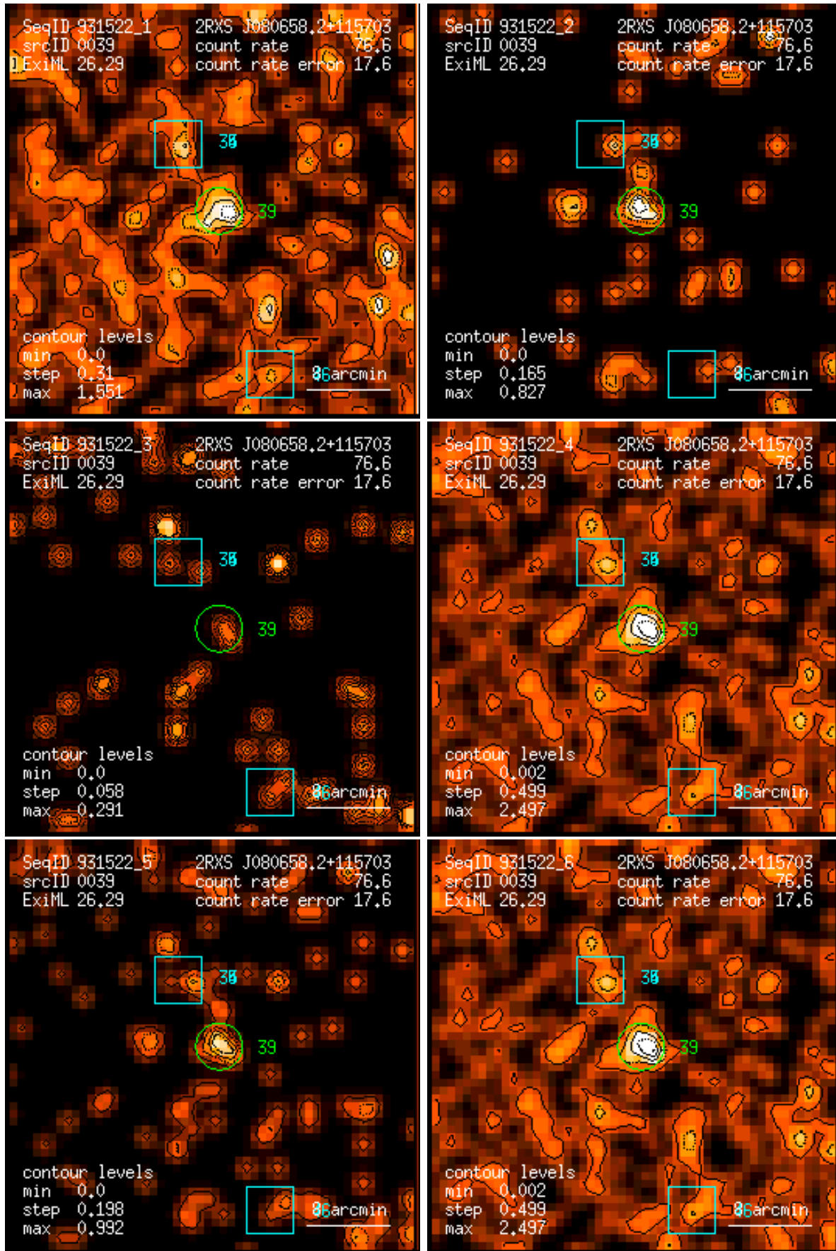
Figure 39: RASS 931522: detection 0039: band rate images, Gaussian filter: (1) PSPC channels 11 – 41, (2) 52 – 90, (3) 91 – 201, (4) 11 – 235, (5) 52 – 201, (6) 11 – 201. Broad band rates in counts/ks. Band rate contour levels in counts/ks/arcmin 2 .
