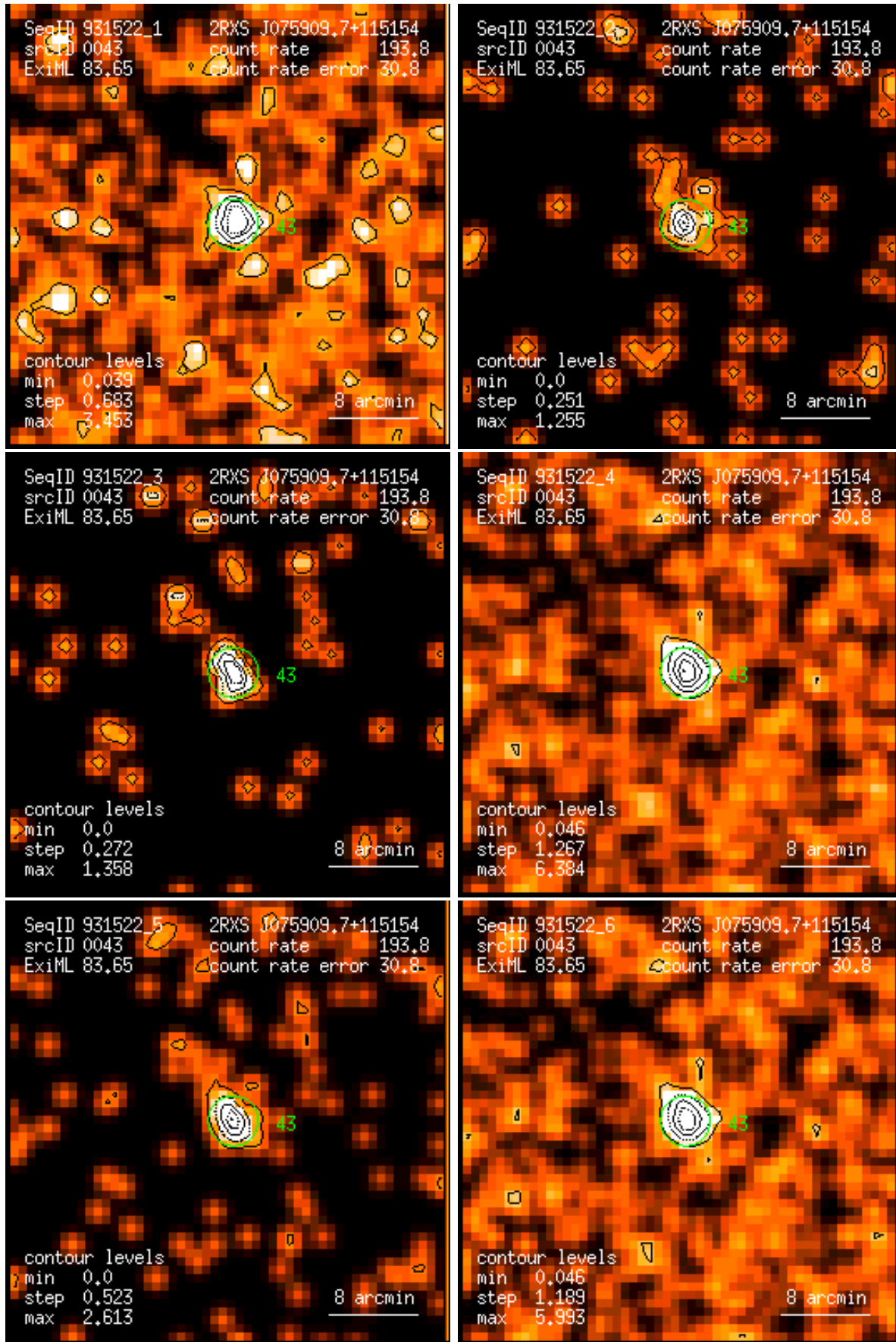
Figure 43: RASS 931522: detection 0043: band rate images, Gaussian filter: (1) PSPC channels 11 – 41, (2) 52 – 90, (3) 91 – 201, (4) 11 – 235, (5) 52 – 201, (6) 11 – 201. Broad band rates in counts/ks. Band rate contour levels in counts/ks/arcmin 2 .
