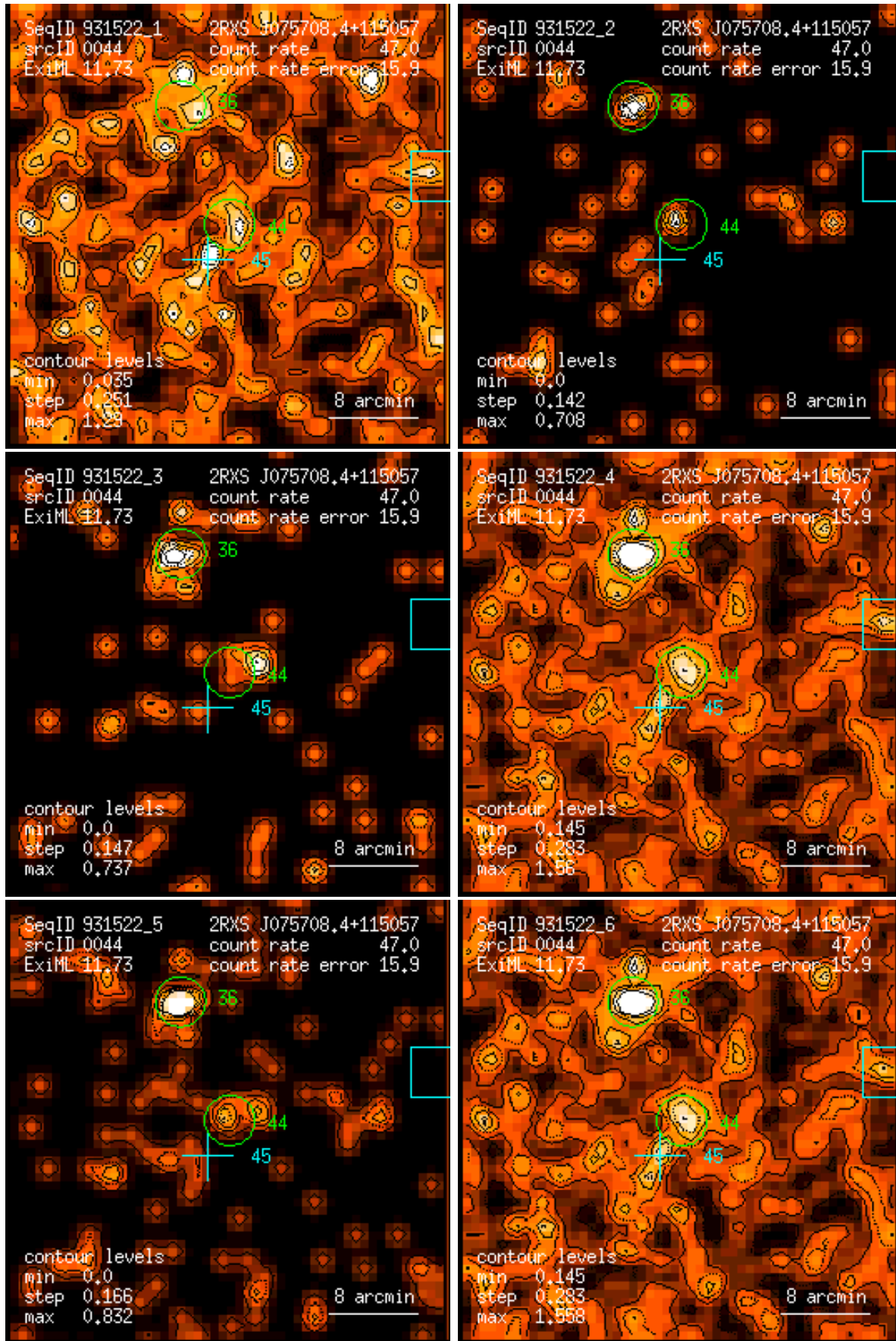
Figure 44: RASS 931522: detection 0044: band rate images, Gaussian filter: (1) PSPC channels 11 – 41, (2) 52 – 90, (3) 91 – 201, (4) 11 – 235, (5) 52 – 201, (6) 11 – 201. Broad band rates in counts/ks. Band rate contour levels in counts/ks/arcmin 2 .
