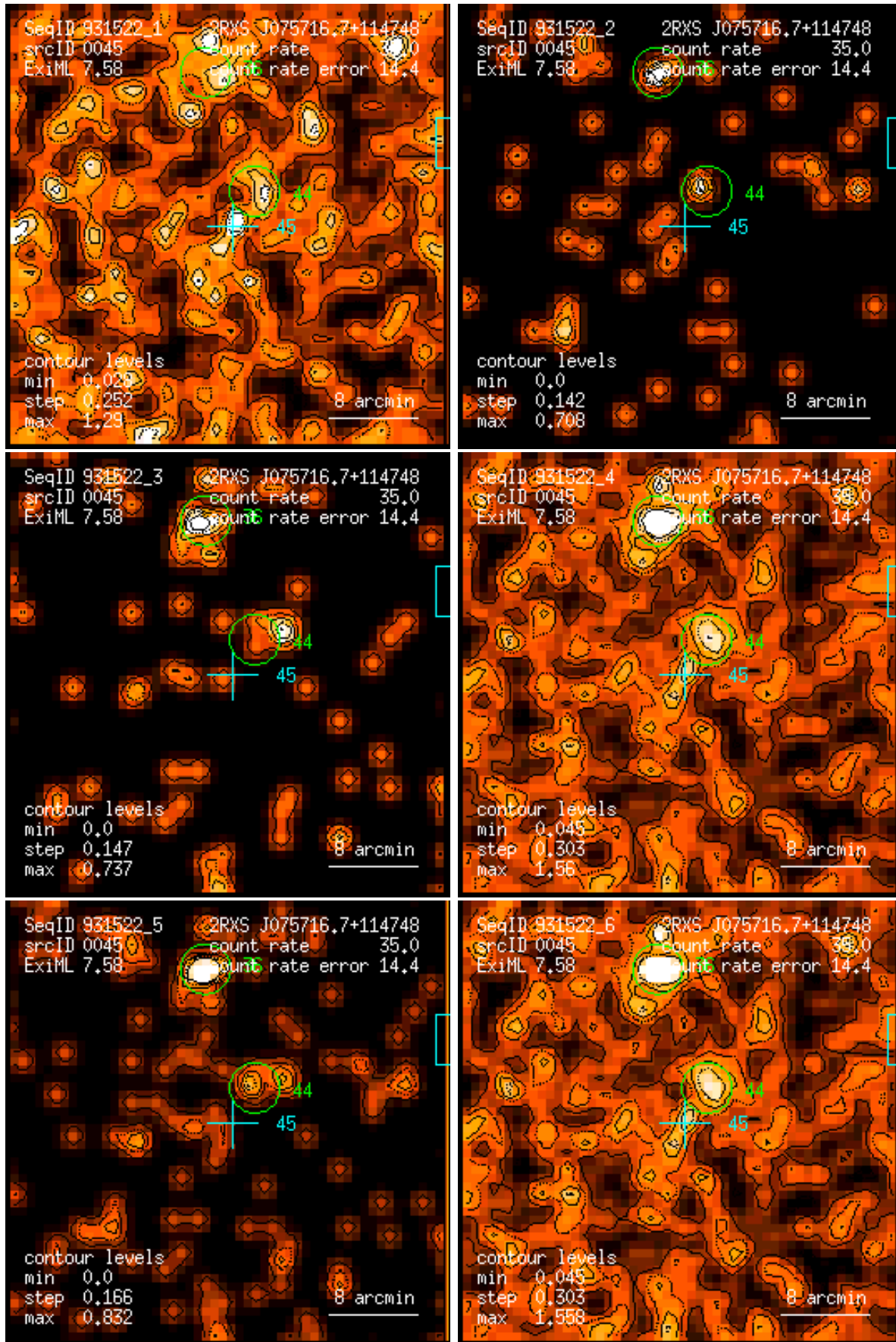
Figure 45: RASS 931522: detection 0045: band rate images, Gaussian filter: (1) PSPC channels 11 – 41, (2) 52 – 90, (3) 91 – 201, (4) 11 – 235, (5) 52 – 201, (6) 11 – 201. Broad band rates in counts/ks. Band rate contour levels in counts/ks/arcmin 2 .
