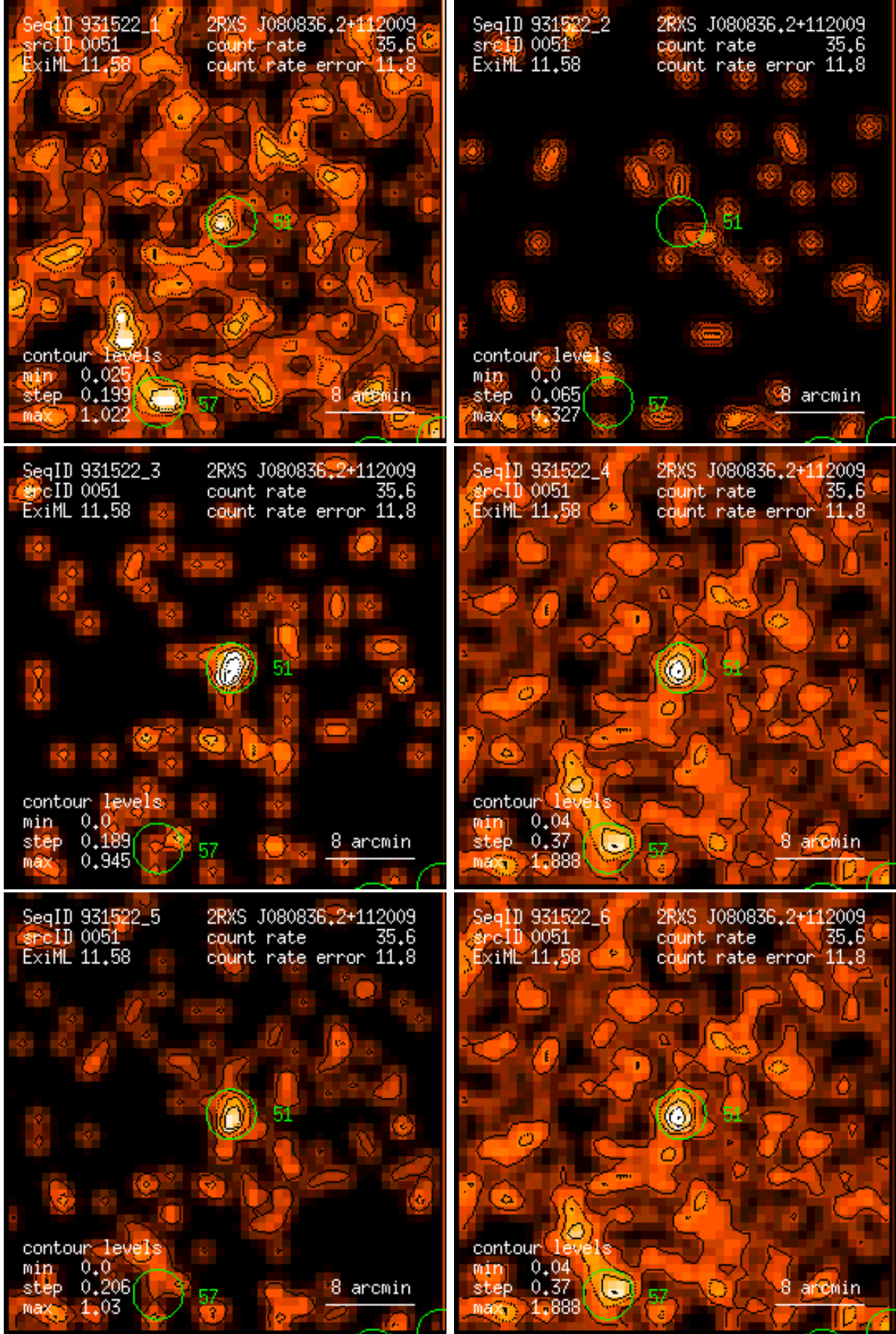
Figure 51: RASS 931522: detection 0051: band rate images, Gaussian filter: (1) PSPC channels 11 – 41, (2) 52 – 90, (3) 91 – 201, (4) 11 – 235, (5) 52 – 201, (6) 11 – 201. Broad band rates in counts/ks. Band rate contour levels in counts/ks/arcmin 2 .
