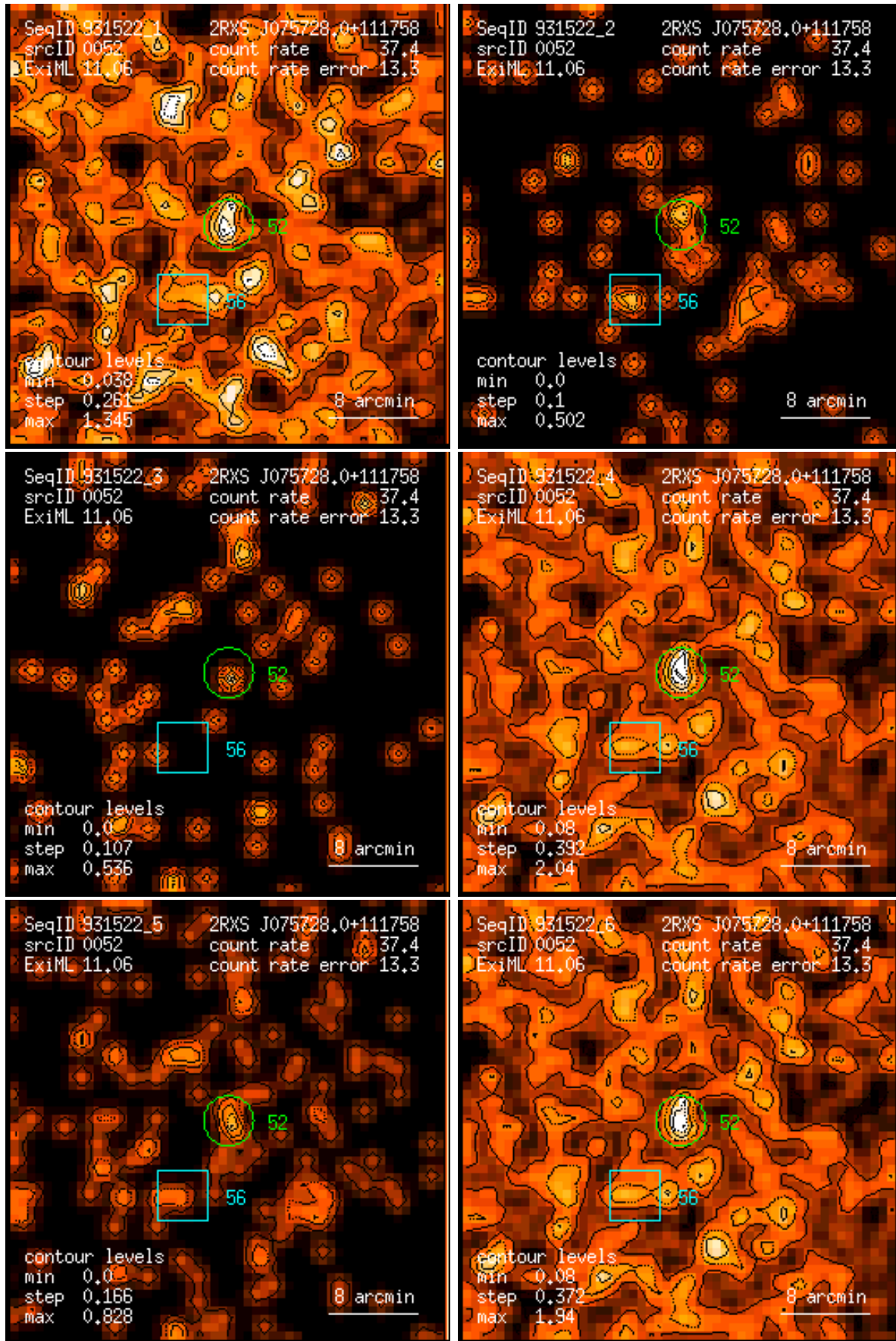
Figure 52: RASS 931522: detection 0052: band rate images, Gaussian filter: (1) PSPC channels 11 – 41, (2) 52 – 90, (3) 91 – 201, (4) 11 – 235, (5) 52 – 201, (6) 11 – 201. Broad band rates in counts/ks. Band rate contour levels in counts/ks/arcmin 2 .
