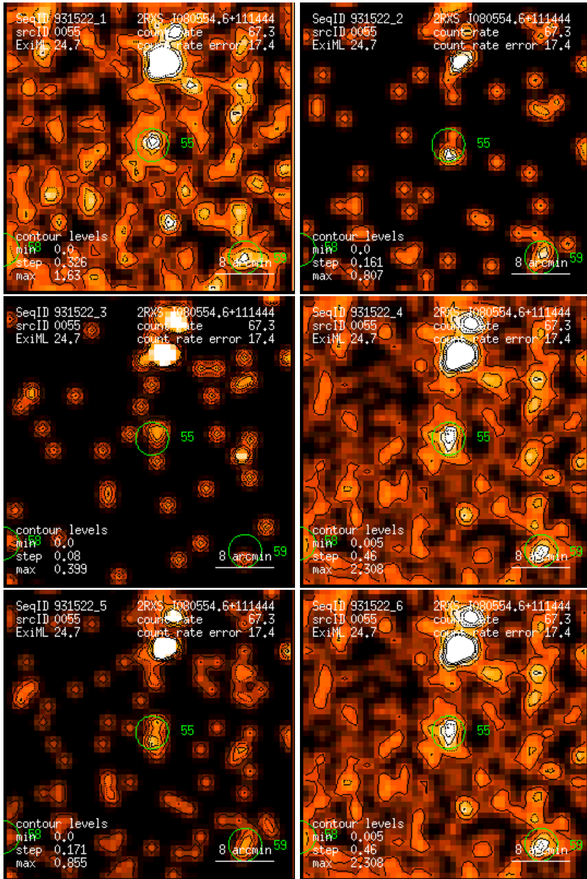
Figure 55: RASS 931522: detection 0055: band rate images, Gaussian filter: (1) PSPC channels 11 – 41, (2) 52 – 90, (3) 91 – 201, (4) 11 – 235, (5) 52 – 201, (6) 11 – 201. Broad band rates in counts/ks. Band rate contour levels in counts/ks/arcmin 2 .
