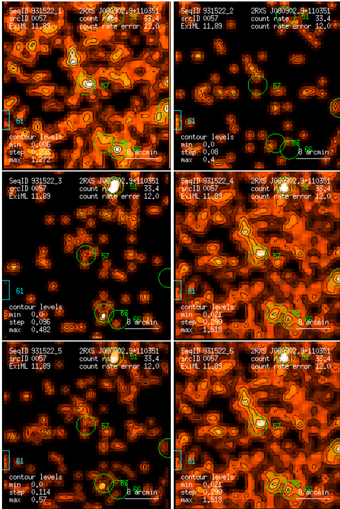
Figure 57: RASS 931522: detection 0057: band rate images, Gaussian filter: (1) PSPC channels 11 – 41, (2) 52 – 90, (3) 91 – 201, (4) 11 – 235, (5) 52 – 201, (6) 11 – 201. Broad band rates in counts/ks. Band rate contour levels in counts/ks/arcmin 2 .
