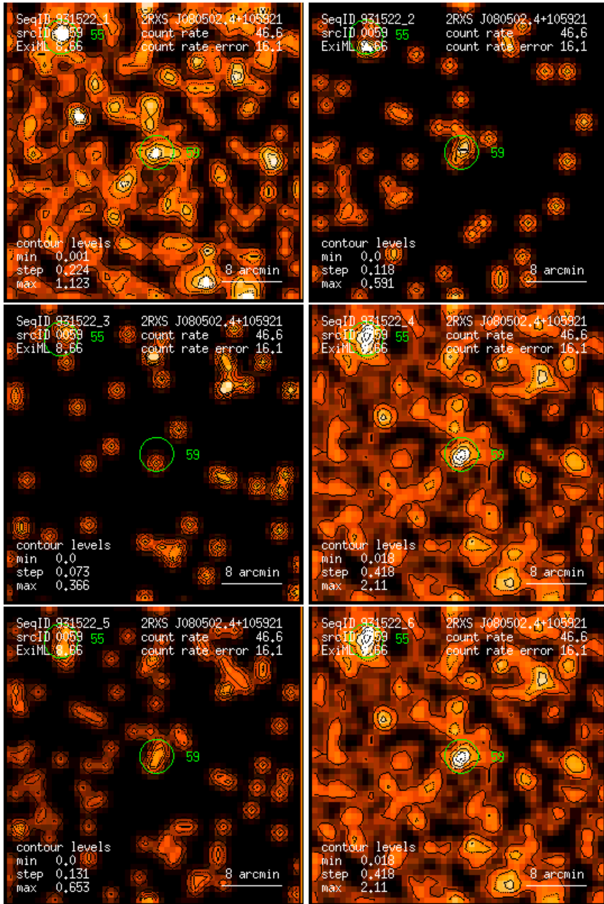
Figure 59: RASS 931522: detection 0059: band rate images, Gaussian filter: (1) PSPC channels 11 – 41, (2) 52 – 90, (3) 91 – 201, (4) 11 – 235, (5) 52 – 201, (6) 11 – 201. Broad band rates in counts/ks. Band rate contour levels in counts/ks/arcmin 2 .
