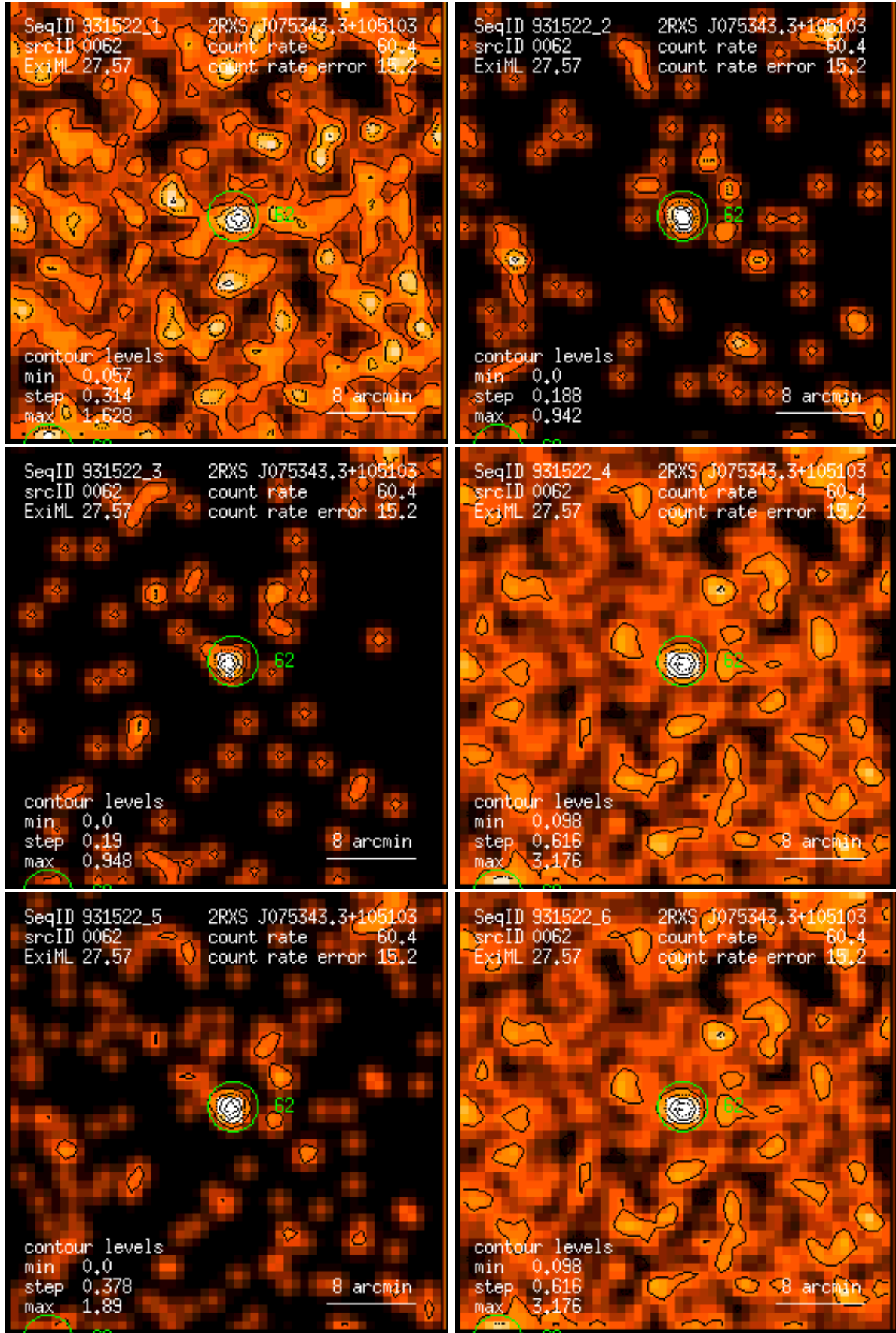
Figure 62: RASS 931522: detection 0062: band rate images, Gaussian filter: (1) PSPC channels 11 – 41, (2) 52 – 90, (3) 91 – 201, (4) 11 – 235, (5) 52 – 201, (6) 11 – 201. Broad band rates in counts/ks. Band rate contour levels in counts/ks/arcmin 2 .
