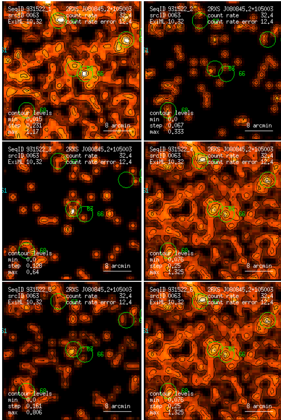
Figure 63: RASS 931522: detection 0063: band rate images, Gaussian filter: (1) PSPC channels 11 – 41, (2) 52 – 90, (3) 91 – 201, (4) 11 – 235, (5) 52 – 201, (6) 11 – 201. Broad band rates in counts/ks. Band rate contour levels in counts/ks/arcmin 2 .
