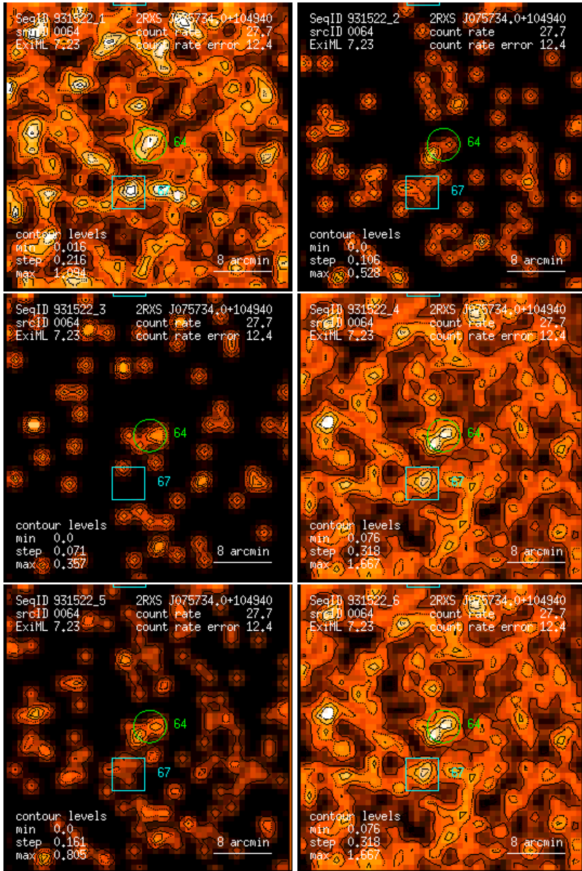
Figure 64: RASS 931522: detection 0064: band rate images, Gaussian filter: (1) PSPC channels 11 – 41, (2) 52 – 90, (3) 91 – 201, (4) 11 – 235, (5) 52 – 201, (6) 11 – 201. Broad band rates in counts/ks. Band rate contour levels in counts/ks/arcmin 2 .
