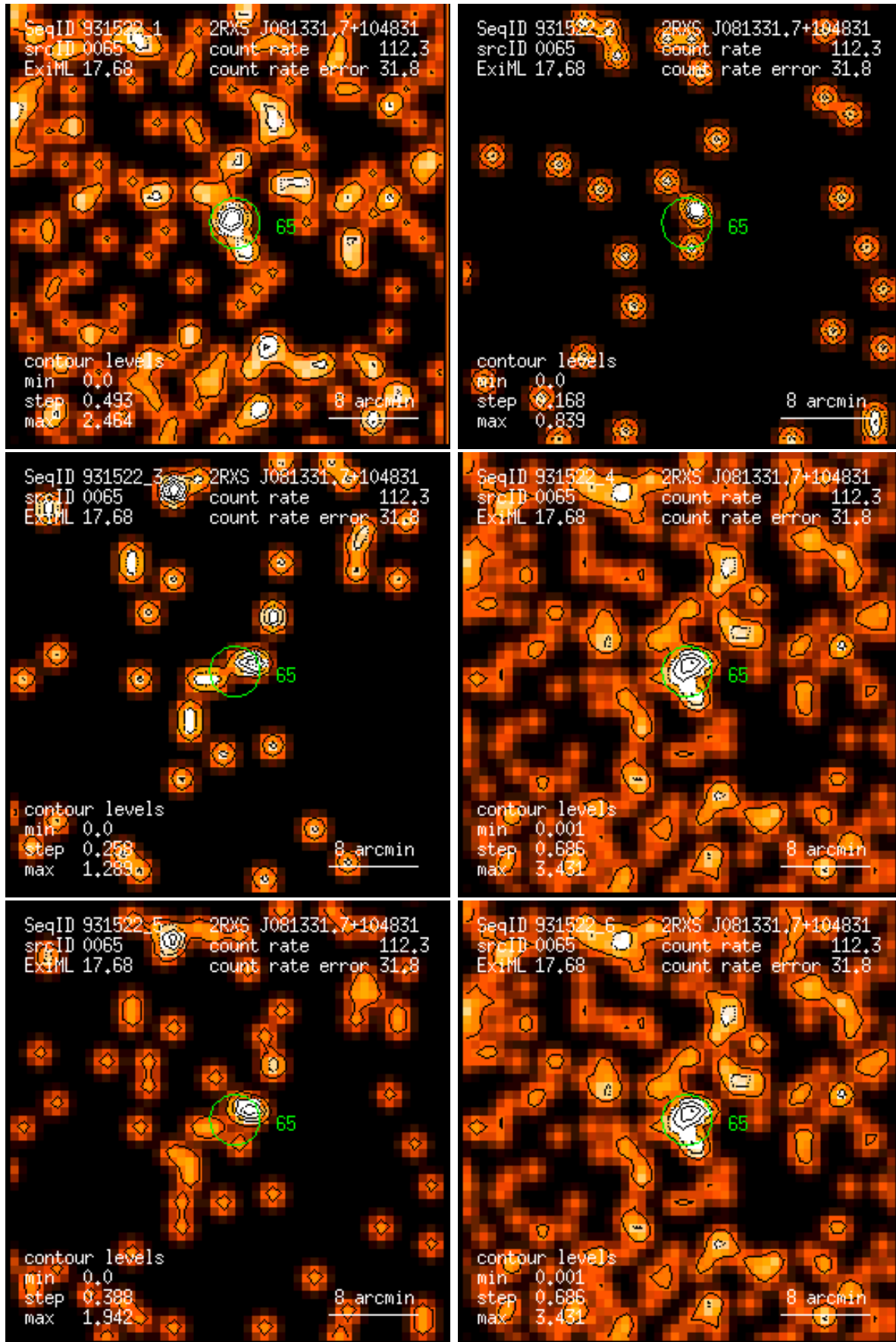
Figure 65: RASS 931522: detection 0065: band rate images, Gaussian filter: (1) PSPC channels 11 – 41, (2) 52 – 90, (3) 91 – 201, (4) 11 – 235, (5) 52 – 201, (6) 11 – 201. Broad band rates in counts/ks. Band rate contour levels in counts/ks/arcmin 2 .
