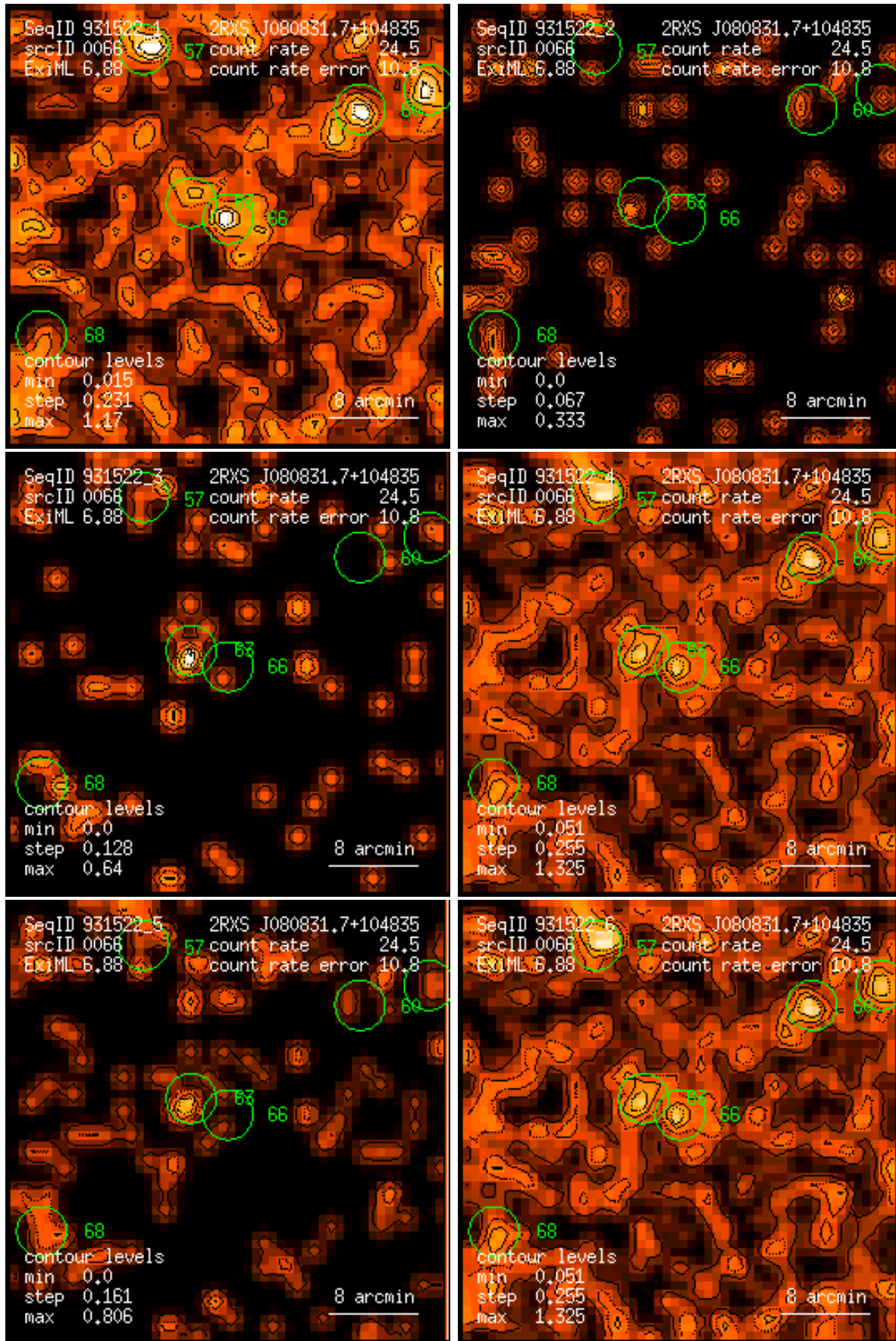
Figure 66: RASS 931522: detection 0066: band rate images, Gaussian filter: (1) PSPC channels 11 – 41, (2) 52 – 90, (3) 91 – 201, (4) 11 – 235, (5) 52 – 201, (6) 11 – 201. Broad band rates in counts/ks. Band rate contour levels in counts/ks/arcmin 2 .
