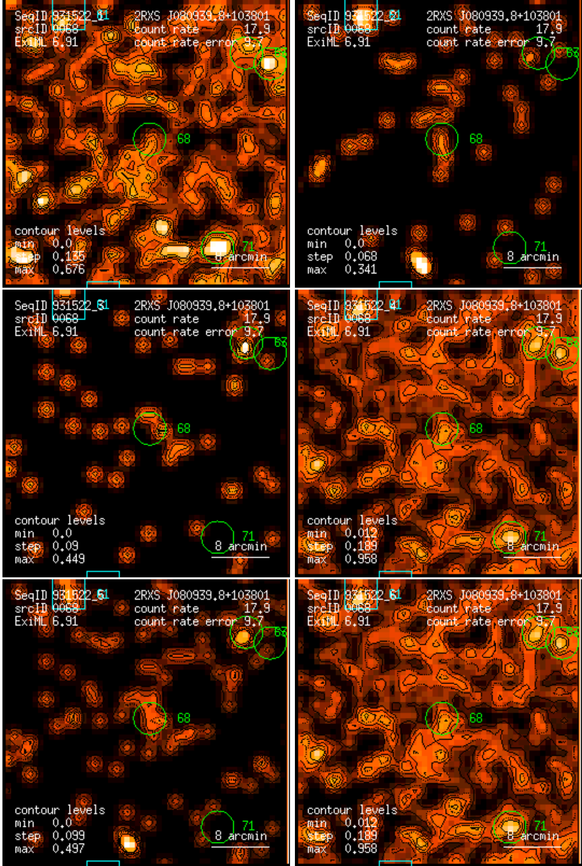
Figure 68: RASS 931522: detection 0068: band rate images, Gaussian filter: (1) PSPC channels 11 – 41, (2) 52 – 90, (3) 91 – 201, (4) 11 – 235, (5) 52 – 201, (6) 11 – 201. Broad band rates in counts/ks. Band rate contour levels in counts/ks/arcmin 2 .
