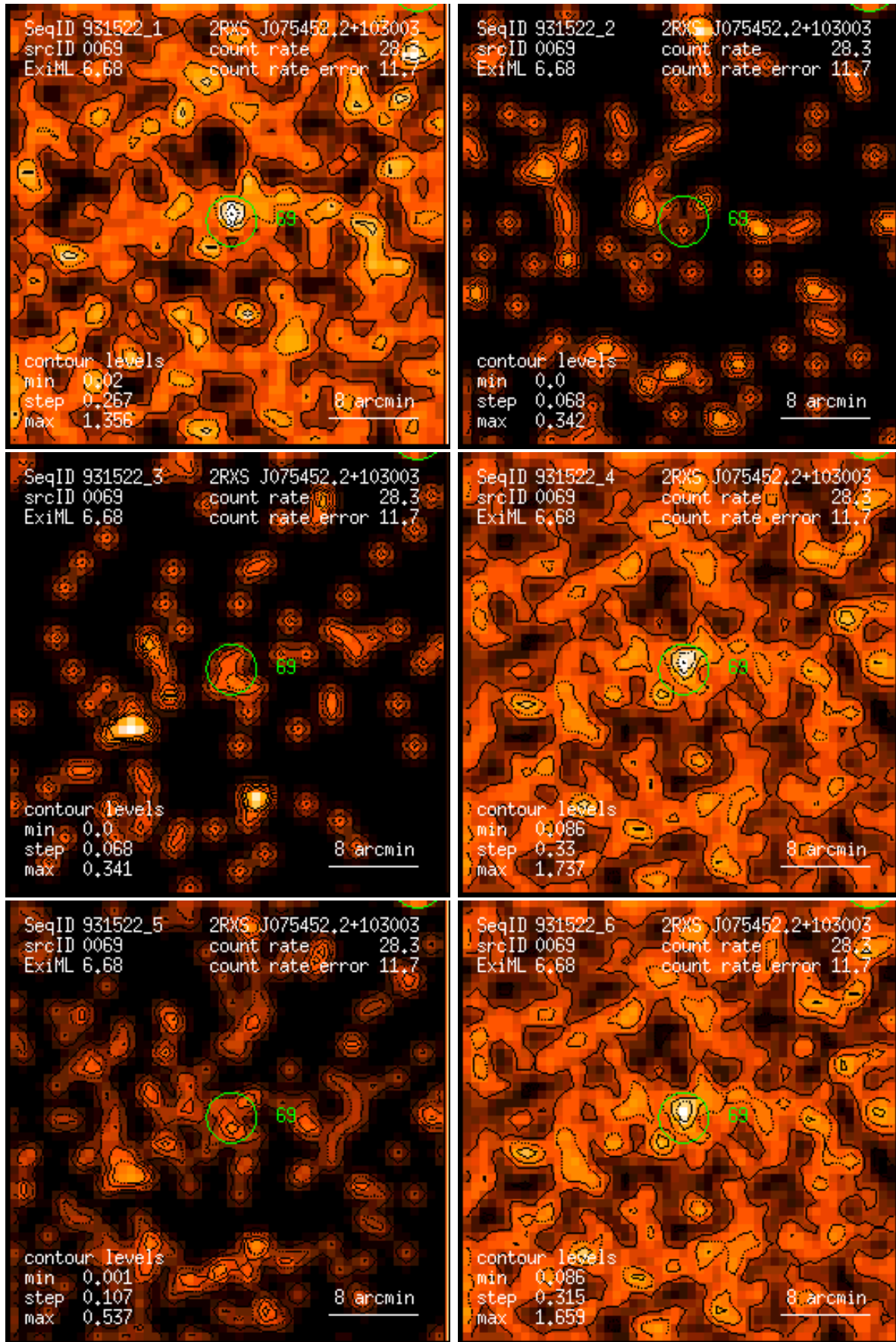
Figure 69: RASS 931522: detection 0069: band rate images, Gaussian filter: (1) PSPC channels 11 – 41, (2) 52 – 90, (3) 91 – 201, (4) 11 – 235, (5) 52 – 201, (6) 11 – 201. Broad band rates in counts/ks. Band rate contour levels in counts/ks/arcmin 2 .
