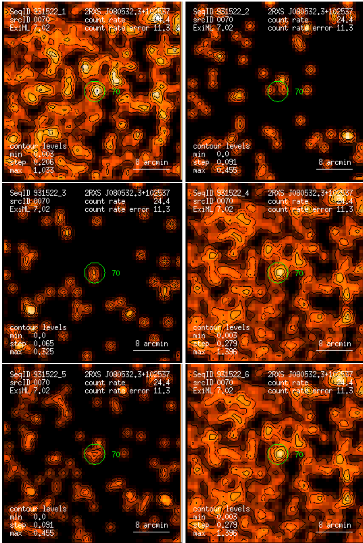
Figure 70: RASS 931522: detection 0070: band rate images, Gaussian filter: (1) PSPC channels 11 – 41, (2) 52 – 90, (3) 91 – 201, (4) 11 – 235, (5) 52 – 201, (6) 11 – 201. Broad band rates in counts/ks. Band rate contour levels in counts/ks/arcmin 2 .
