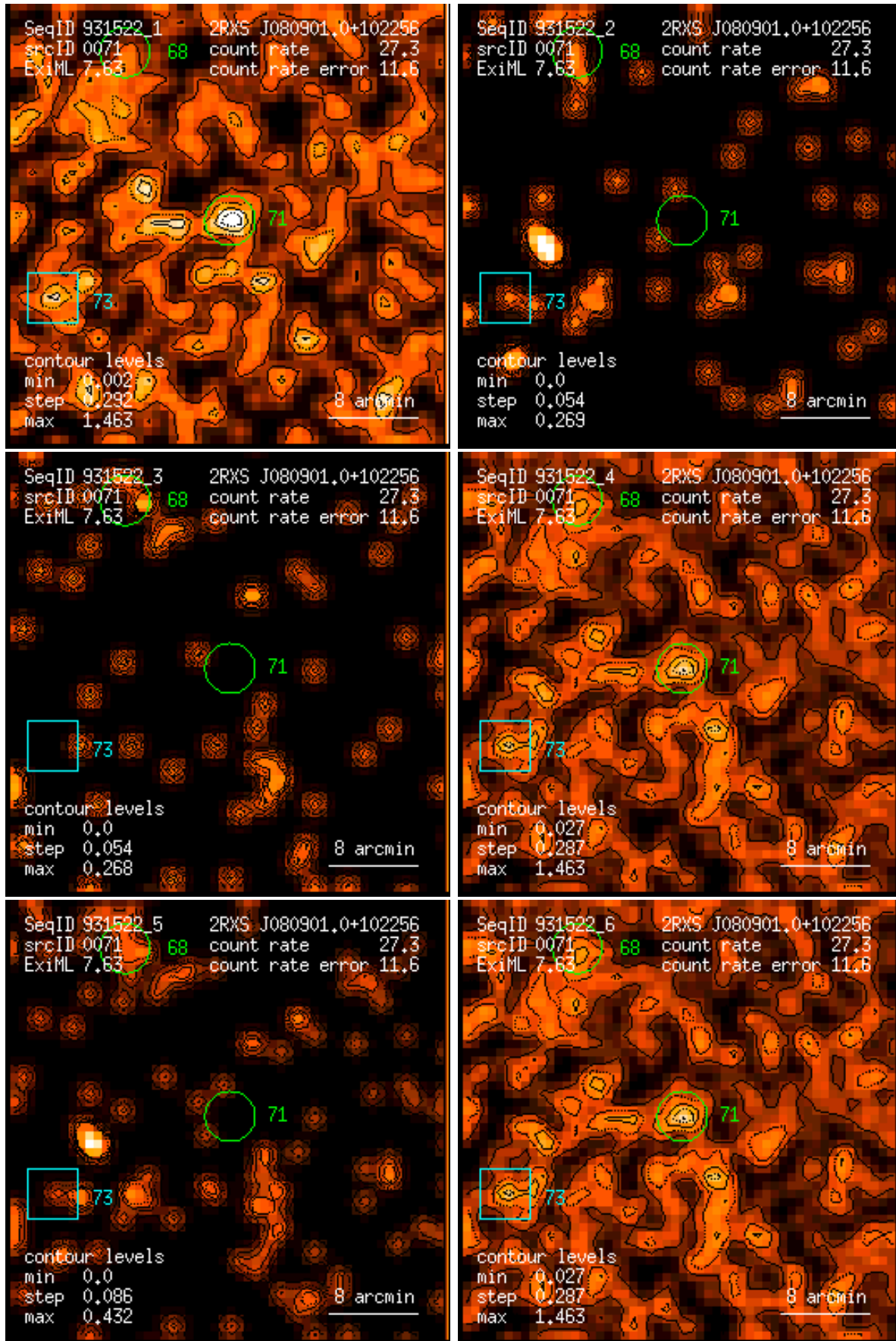
Figure 71: RASS 931522: detection 0071: band rate images, Gaussian filter: (1) PSPC channels 11 – 41, (2) 52 – 90, (3) 91 – 201, (4) 11 – 235, (5) 52 – 201, (6) 11 – 201. Broad band rates in counts/ks. Band rate contour levels in counts/ks/arcmin 2 .
