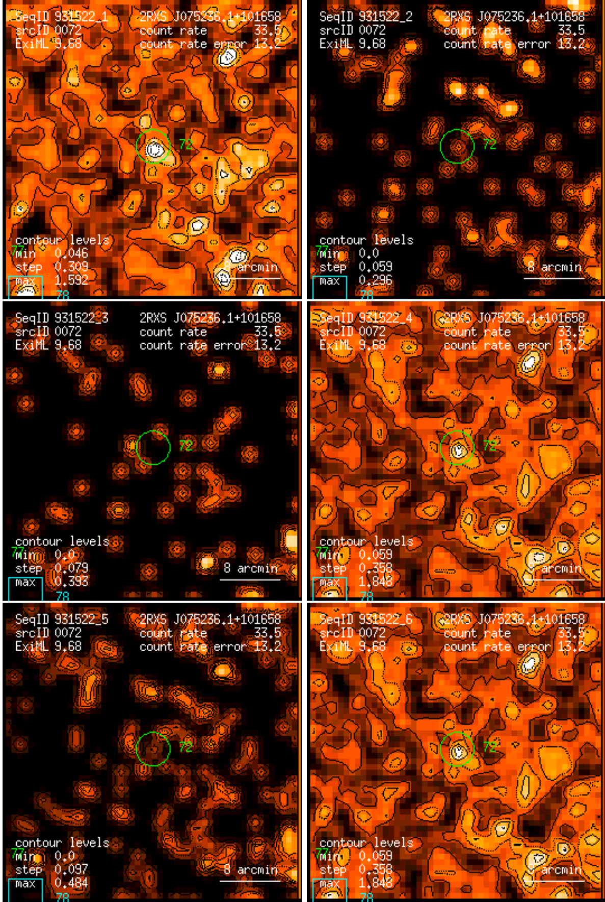
Figure 72: RASS 931522: detection 0072: band rate images, Gaussian filter: (1) PSPC channels 11 – 41, (2) 52 – 90, (3) 91 – 201, (4) 11 – 235, (5) 52 – 201, (6) 11 – 201. Broad band rates in counts/ks. Band rate contour levels in counts/ks/arcmin 2 .
