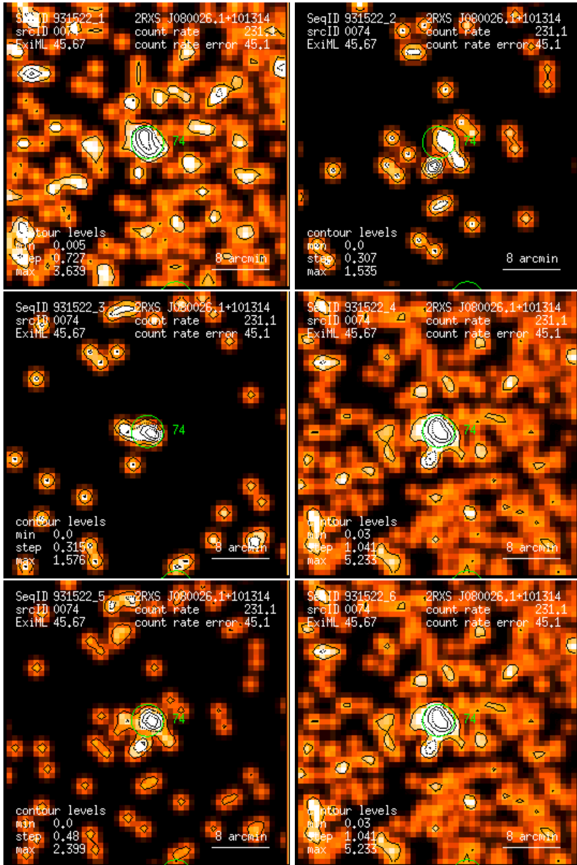
Figure 74: RASS 931522: detection 0074: band rate images, Gaussian filter: (1) PSPC channels 11 – 41, (2) 52 – 90, (3) 91 – 201, (4) 11 – 235, (5) 52 – 201, (6) 11 – 201. Broad band rates in counts/ks. Band rate contour levels in counts/ks/arcmin 2 .
