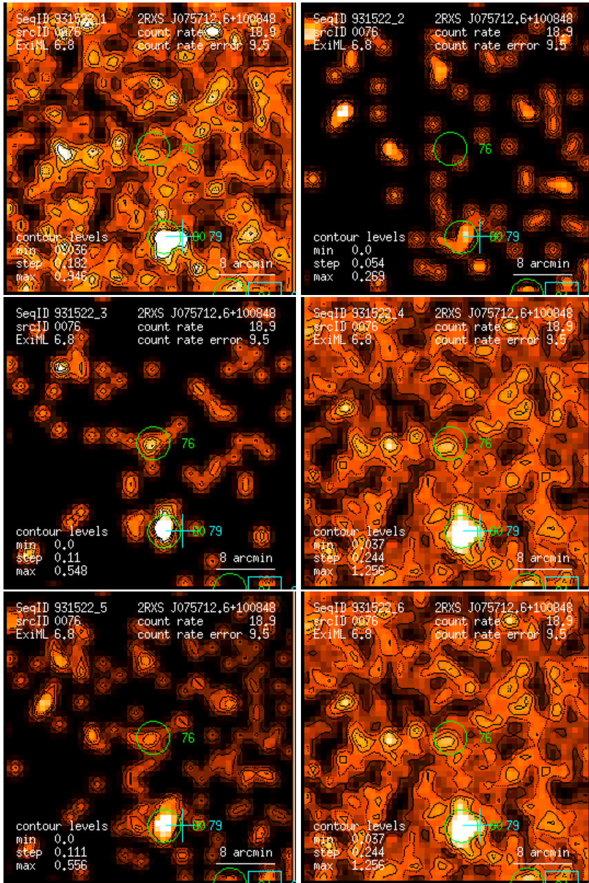
Figure 76: RASS 931522: detection 0076: band rate images, Gaussian filter: (1) PSPC channels 11 – 41, (2) 52 – 90, (3) 91 – 201, (4) 11 – 235, (5) 52 – 201, (6) 11 – 201. Broad band rates in counts/ks. Band rate contour levels in counts/ks/arcmin 2 .
