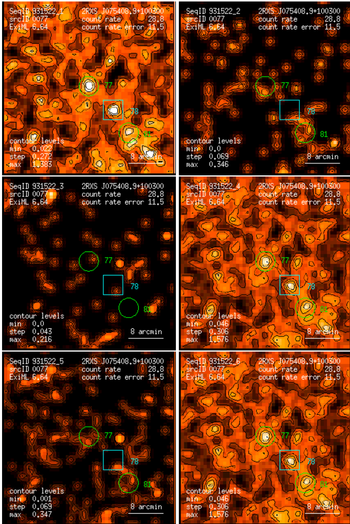
Figure 77: RASS 931522: detection 0077: band rate images, Gaussian filter: (1) PSPC channels 11 – 41, (2) 52 – 90, (3) 91 – 201, (4) 11 – 235, (5) 52 – 201, (6) 11 – 201. Broad band rates in counts/ks. Band rate contour levels in counts/ks/arcmin 2 .
